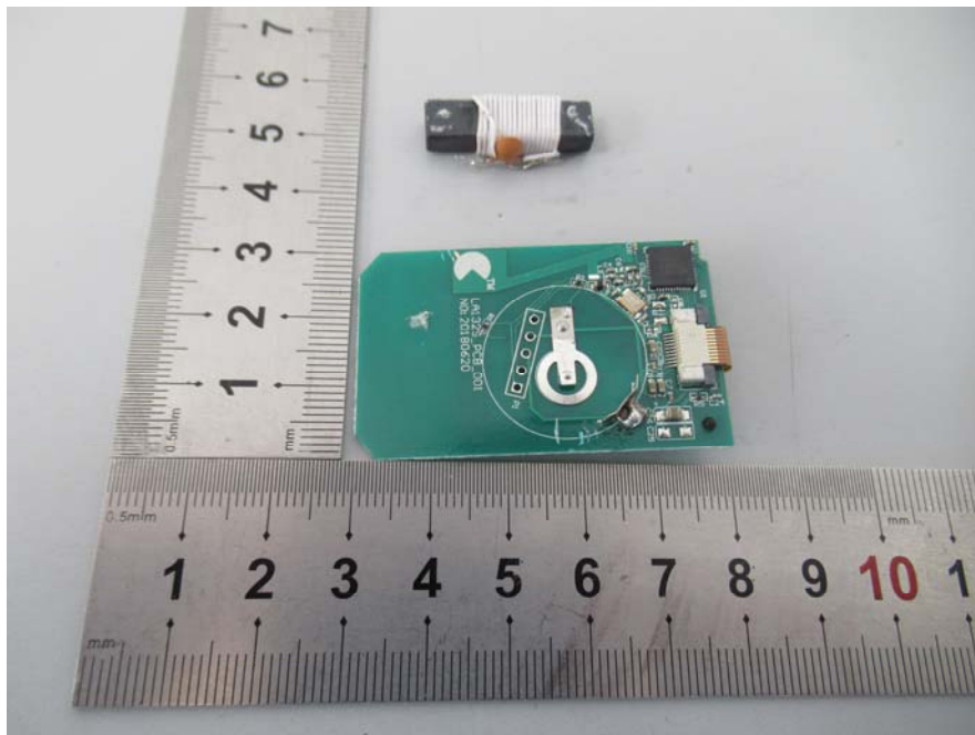
EUT – Magnet View
