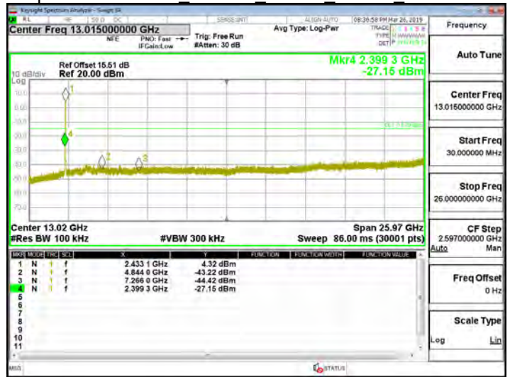
Spurious Emission 802.11n 40MHz Chain0 2437MHz
