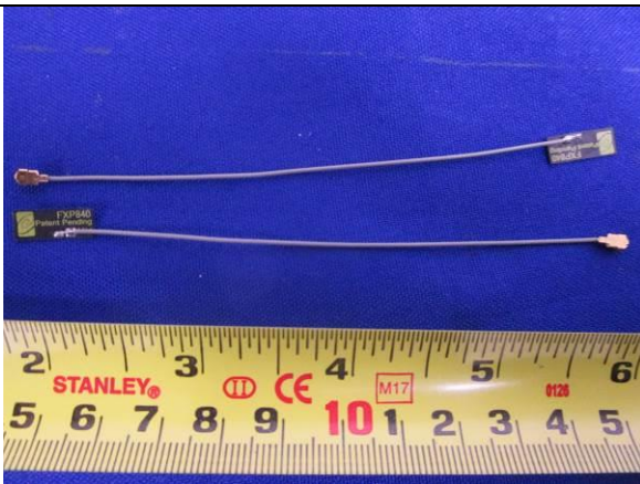
Taoglas FXP840.07.0055B Monopole Antenna- Top View
