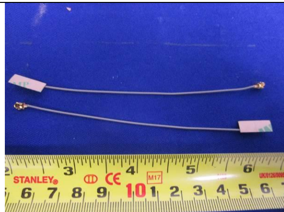
Taoglas FXP840.07.0055B Monopole Antenna – Bottom View
