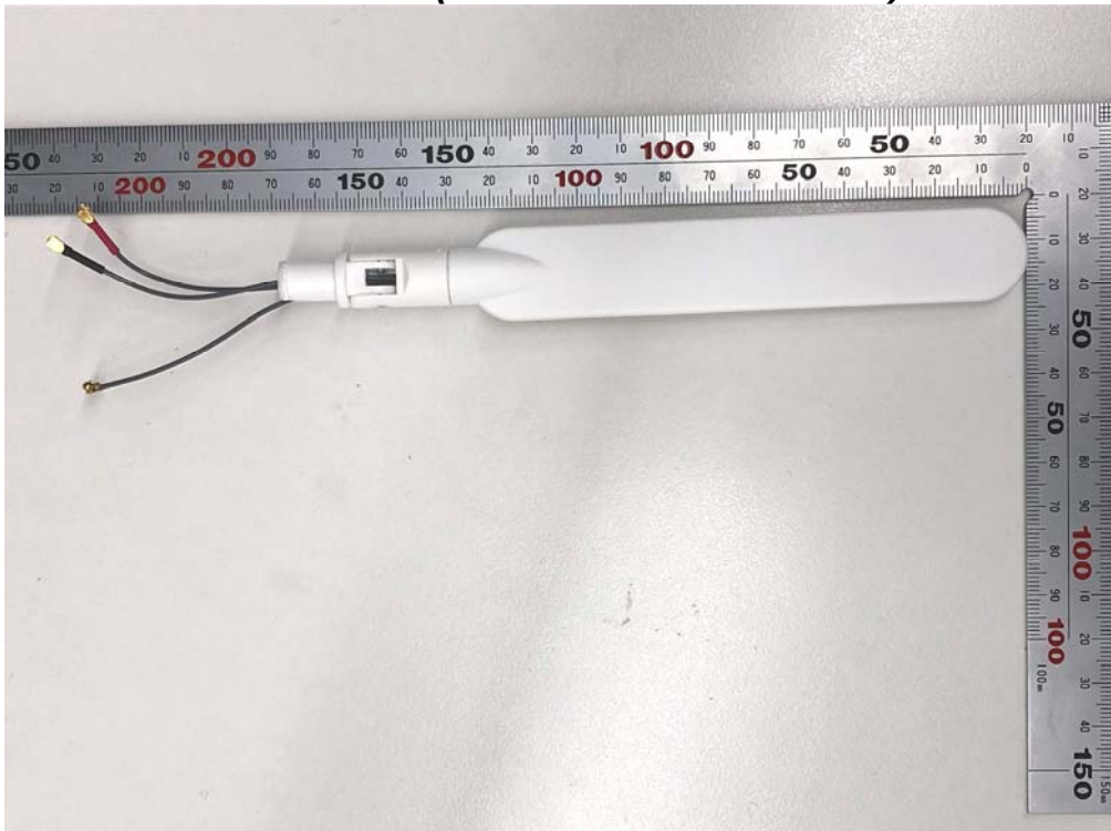
Antenna – 4 (Part No.: KWM-619BMPXX)
