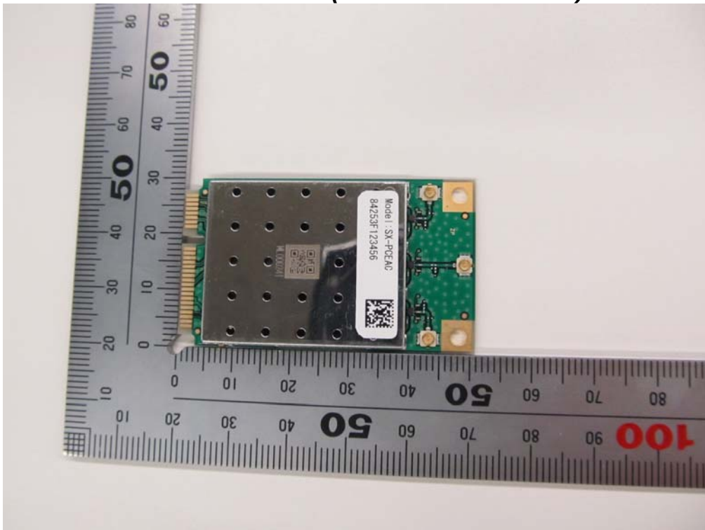
Front View of EUT (Model No.: SX-PCEAC)
