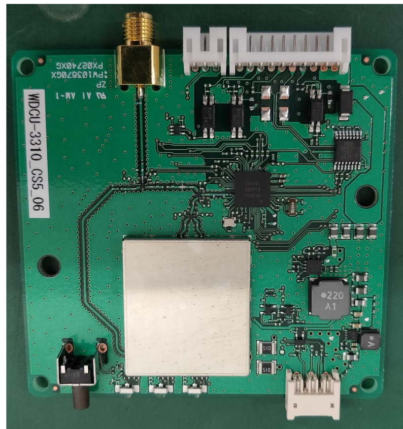
After mounting shield
