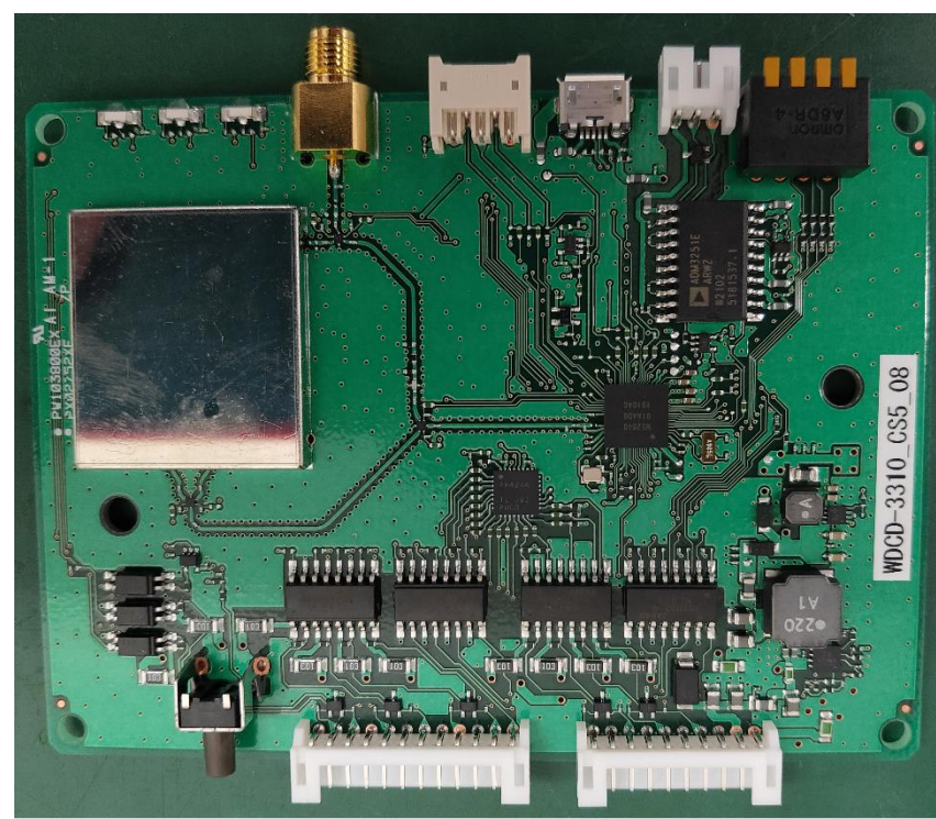
After mounting shield
