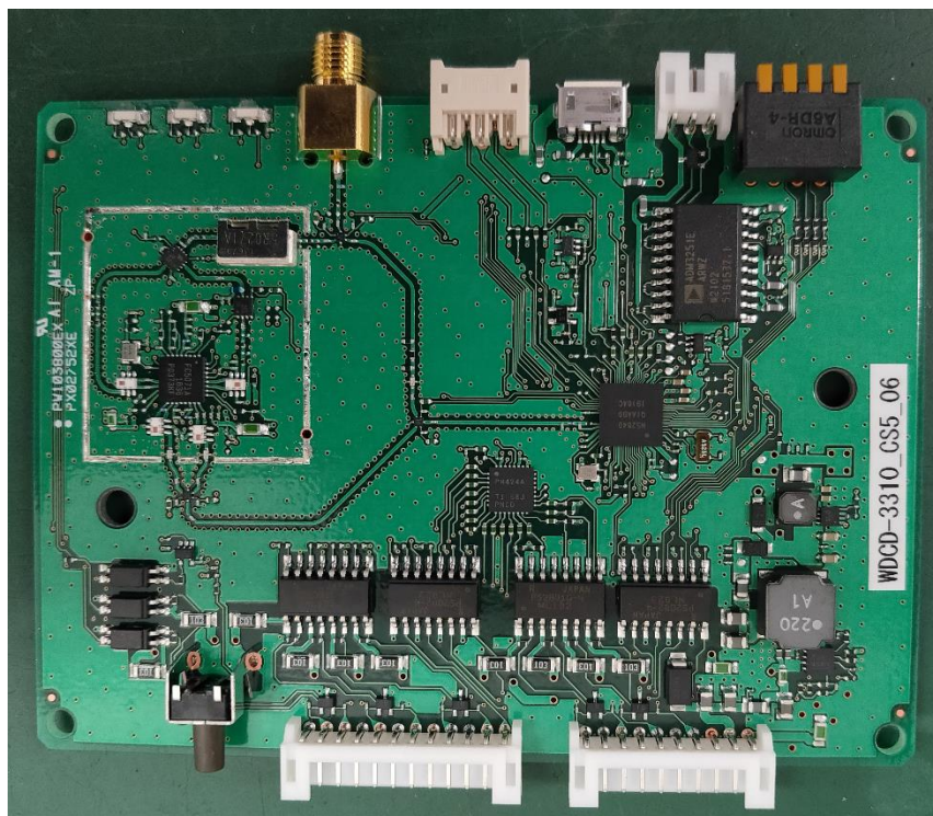
Before mounting shield
