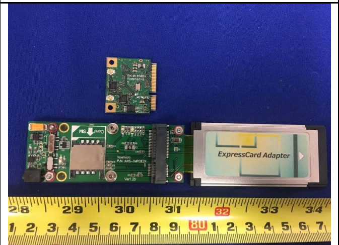
EUT - Module Separation View
