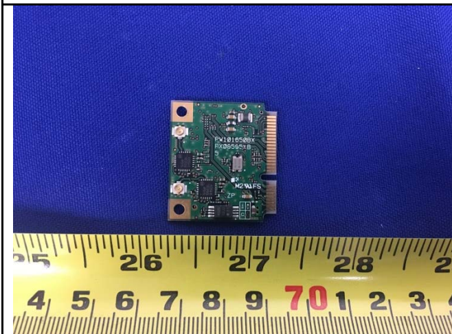
Module - Front View
