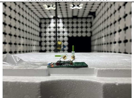
EUT Setup Close View - Back
