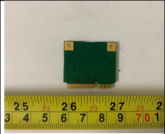
EUT Bottom View
