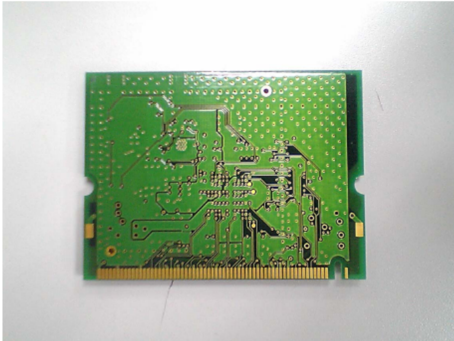
Solder side
