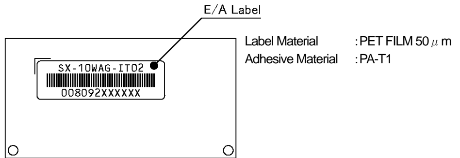
Bottom View
