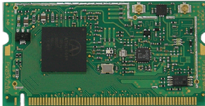
Module Board Side A without Shield
