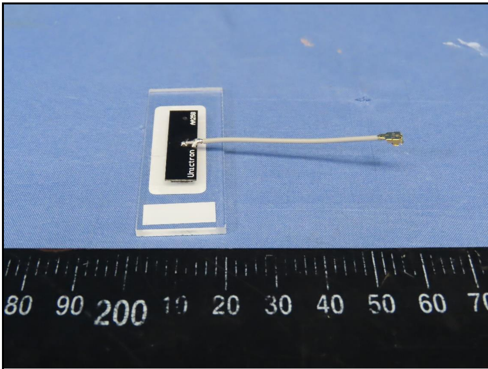
Antenna front
