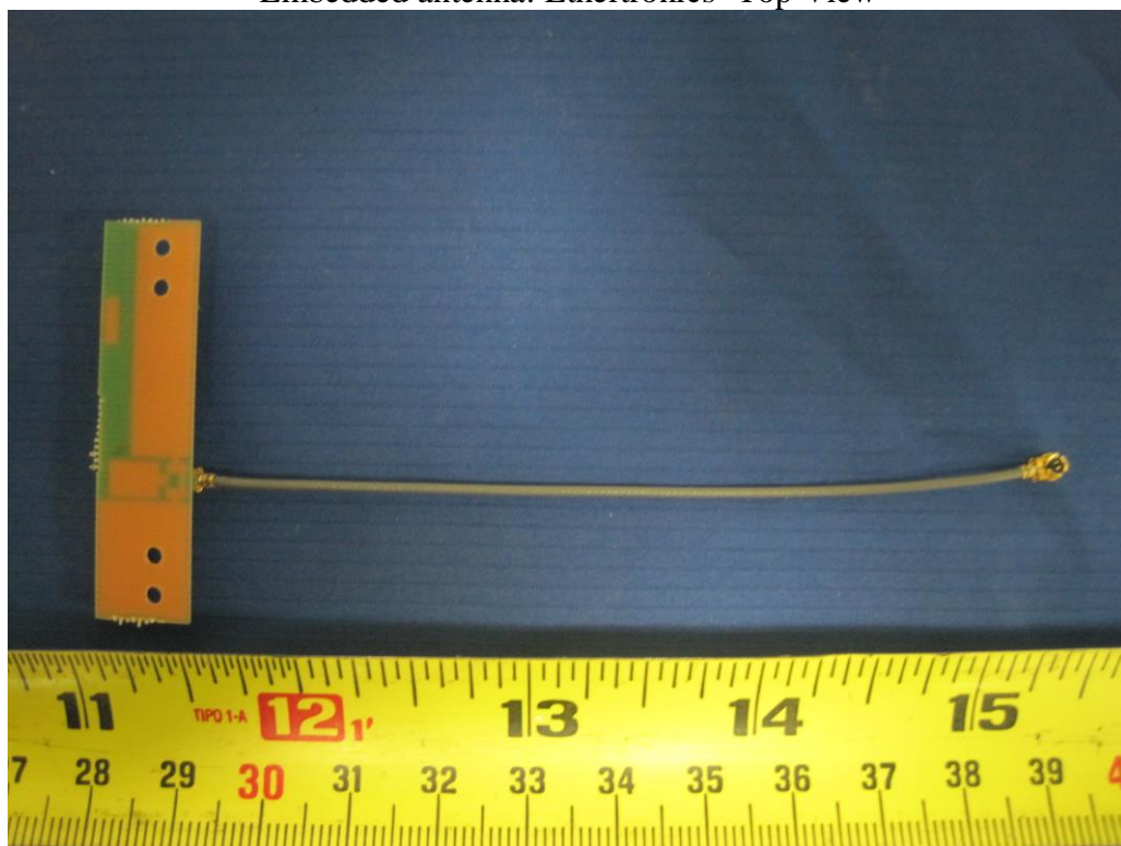
Embedded antenna: Ethertronics -Bottom View
