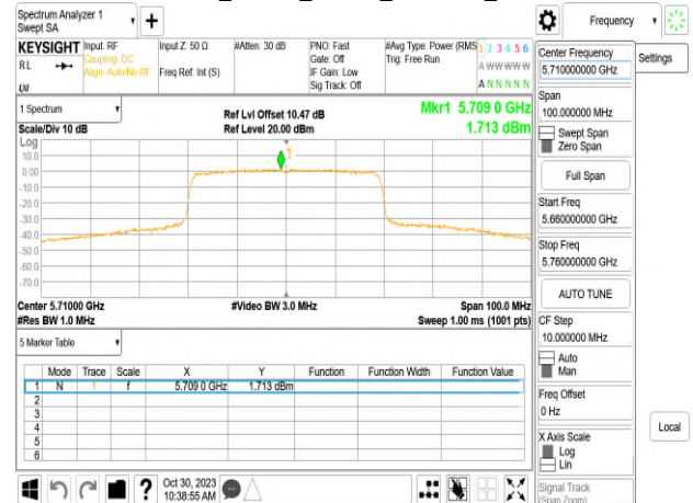
802.11ax_40MHz_Chain0_5710MHz_UNII 2C
