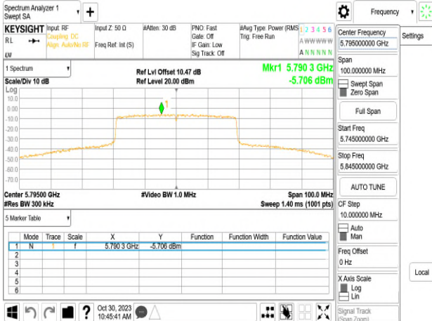
802.11ax_40MHz_Chain0_5795MHz
