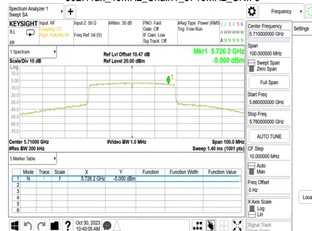
802.11ax_40MHz_Chain1_5710MHz_UNII 3
