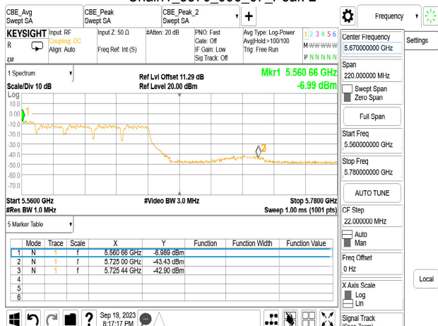
Chain1_5570_996_67_Peak
