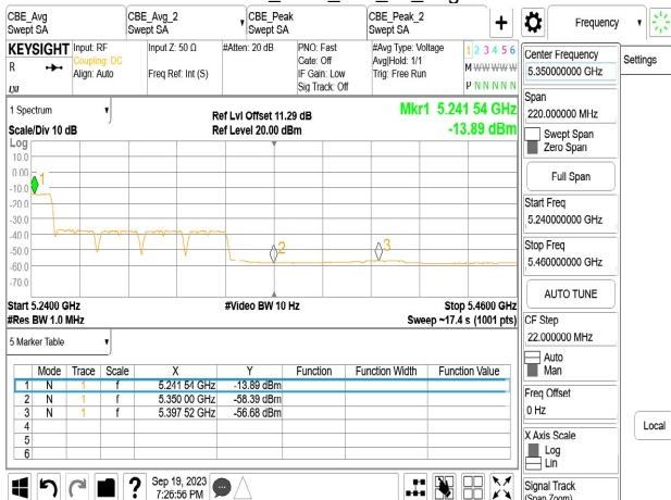
Chain1_5250_996_67_Avg
