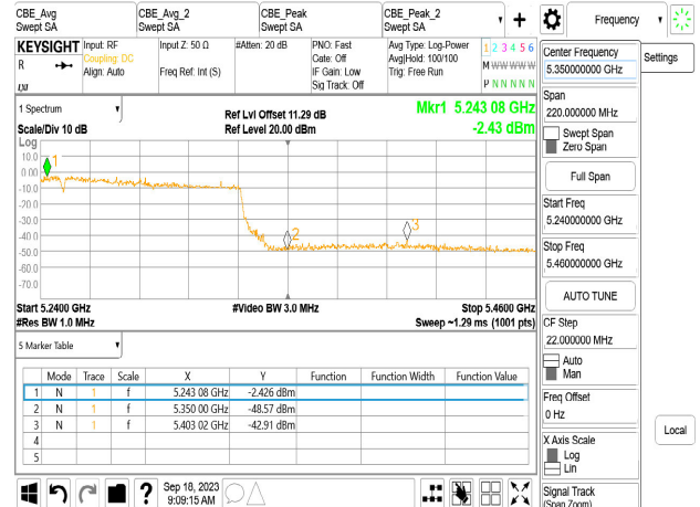
Chain1_5250_Peak
