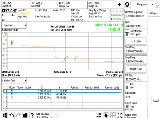
Chain1_5250_Avg-2
