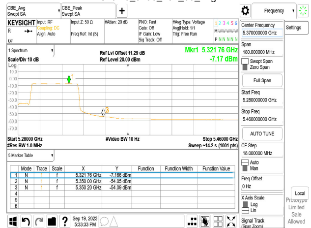
Chain0_5290_484_66_Peak
