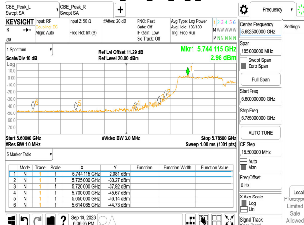
Chain0_5775_484_65_R_Peak
