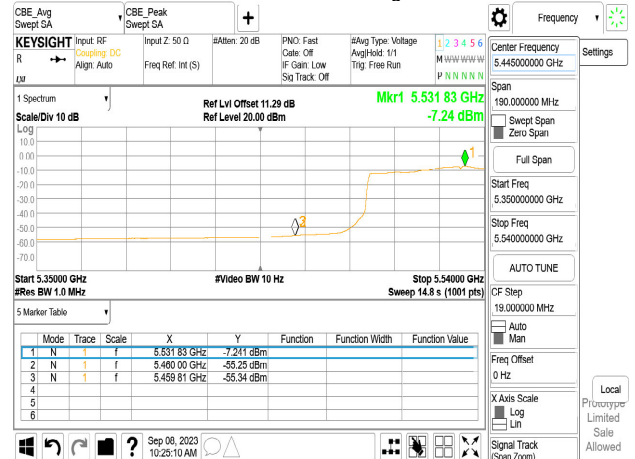
Chain0_5530_Peak
