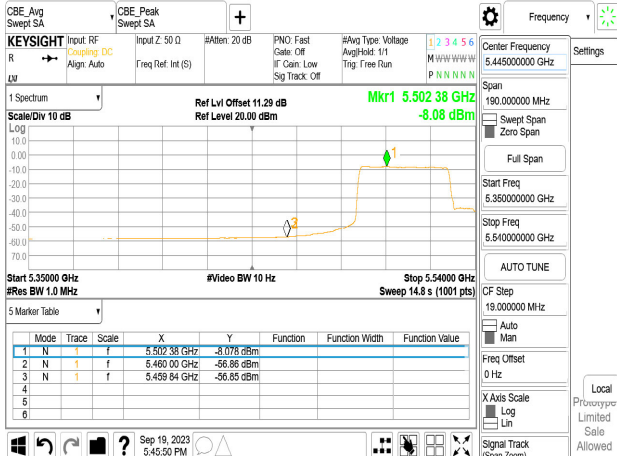
Chain0_5530_484_65_Avg
