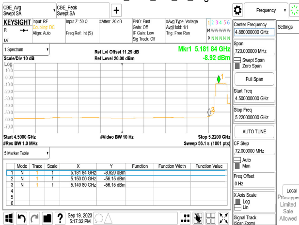
Chain0_5210_484_65_Peak
