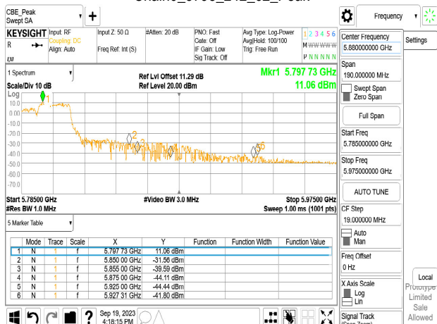
Chain0_5795_Peak
