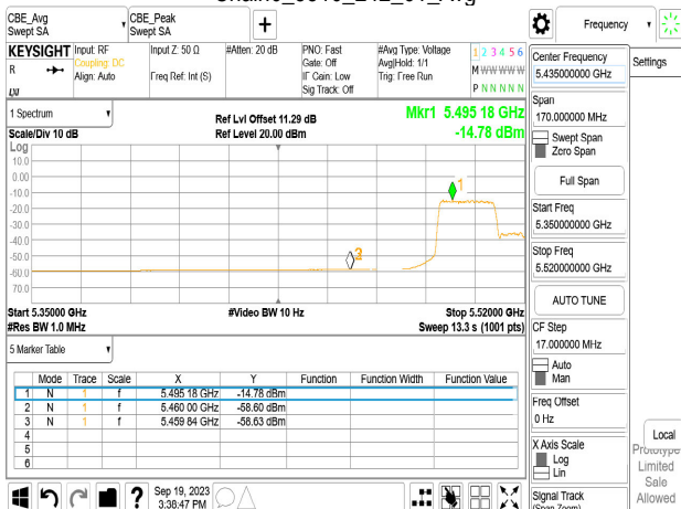
Chain0_5510_242_61_Avg
