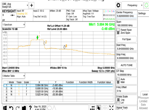
Chain0_5875_242_62_Avg
