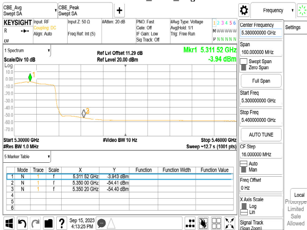
Chain0_5310_Peak
