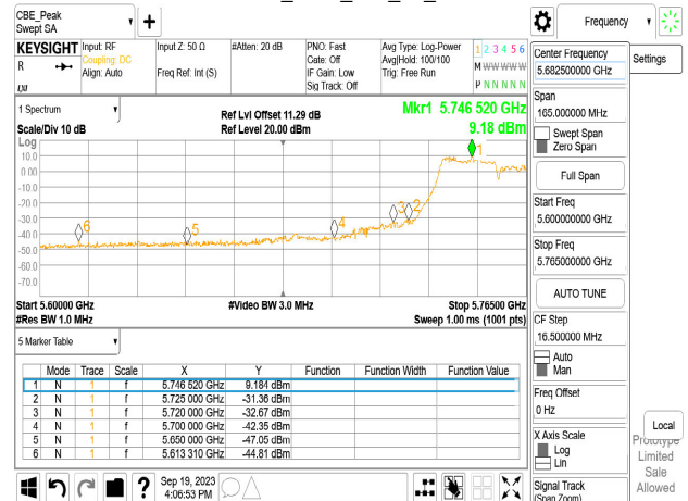
Chain0_5755_Peak
