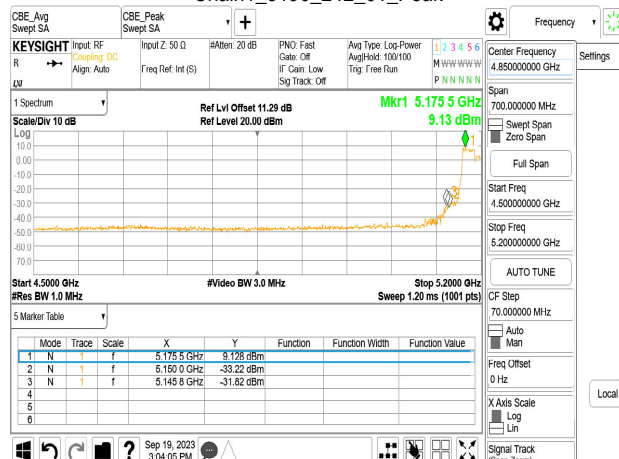
Chain1_5190_242_61_Peak
