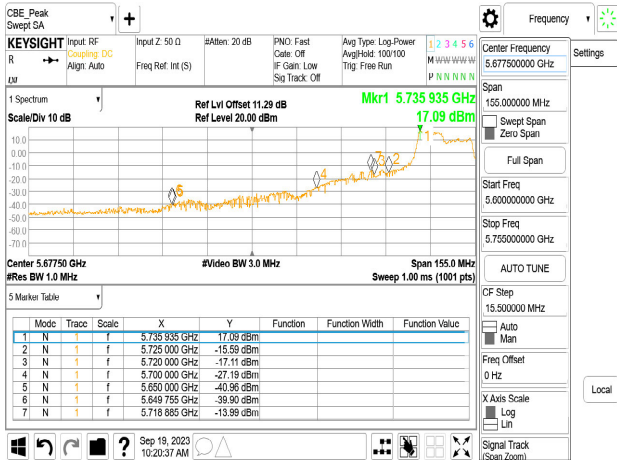
Chain1_5745_26_0_Peak
