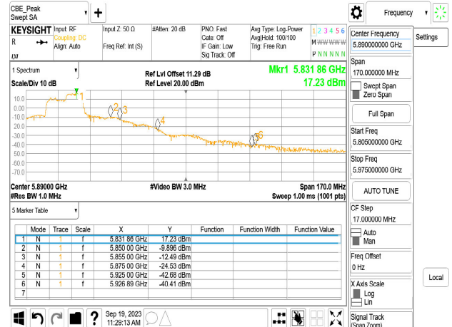
Chain1_5825_26_8_Peak
