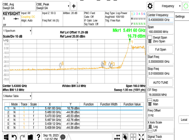
Chain1_5500_52_37_Avg
