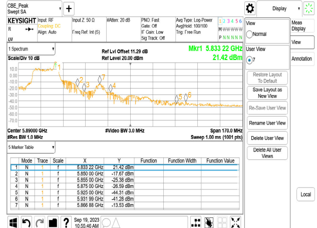
Chain1_5825_26_8_Peak
