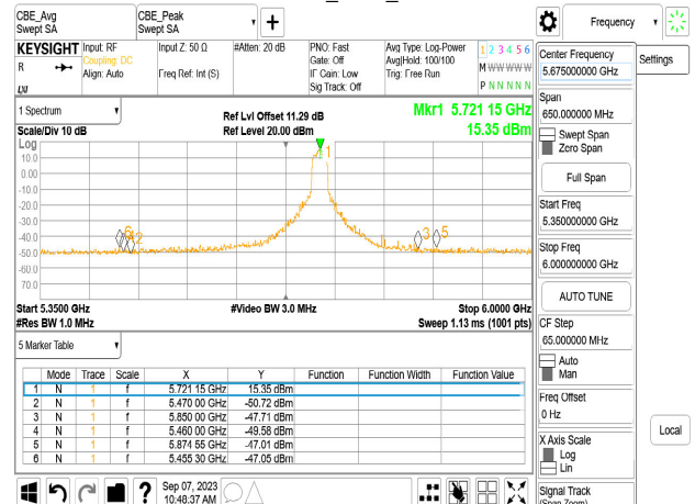
Chain1_5720_Peak
