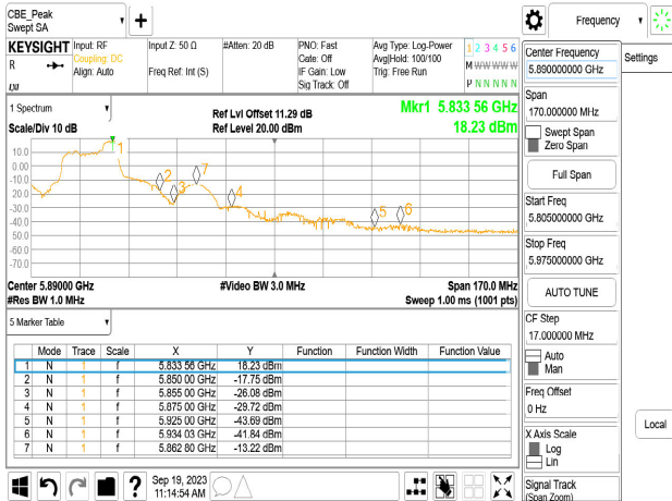
Chain1_5825_Peak
