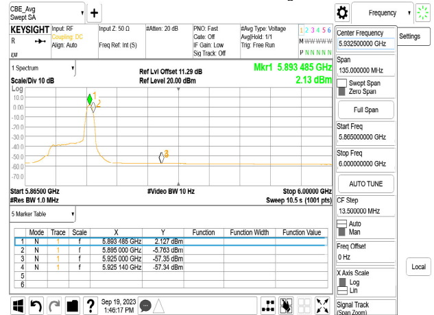
Chain1_5885_52_40_Avg
