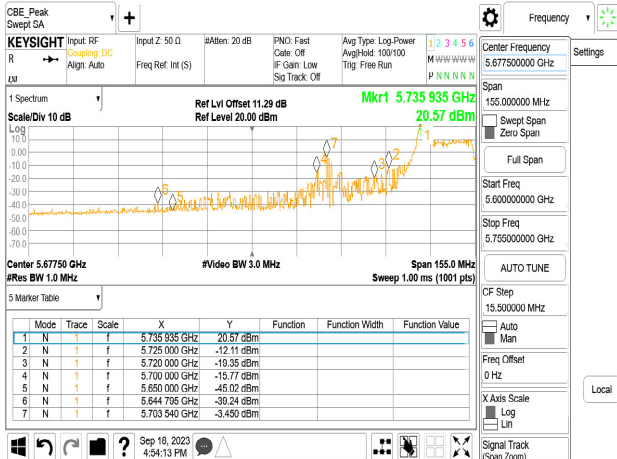
Chain1_5745_52_37_Peak
