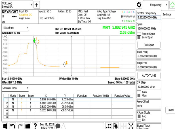
Chain1_5885_106_54_Avg
