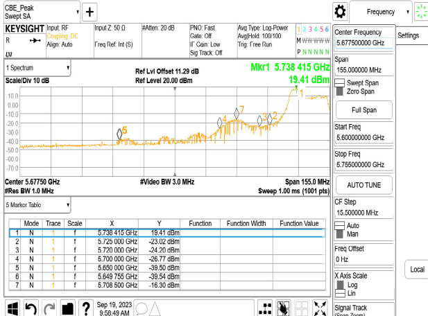
Chain1_5745_52_37_Peak
