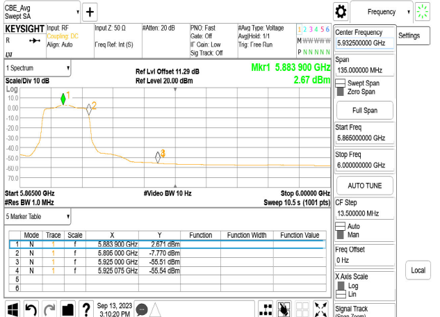
Chain1_5885_Avg
