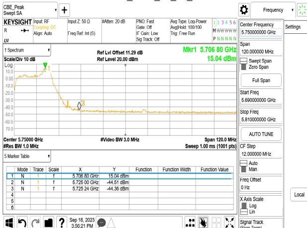
Chain1_5700_52_40_Peak
