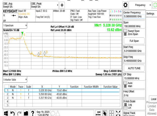
Chain0_5320_26_8_Peak
