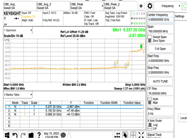
Chain1_5250_Peak_R
