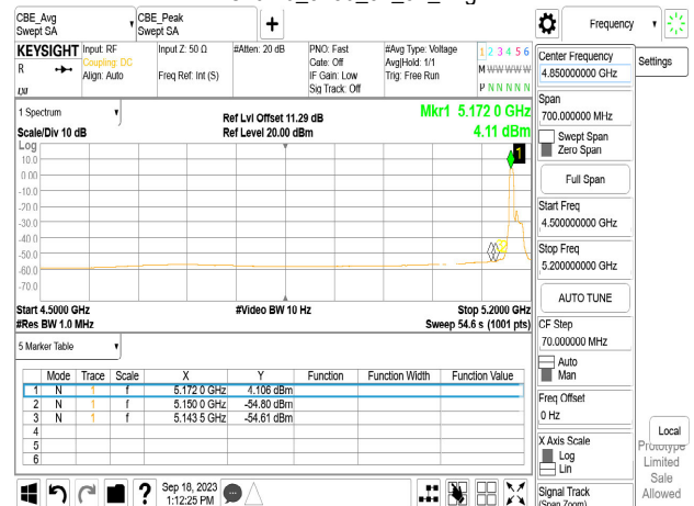
Chain0_5180_52_37_Peak
