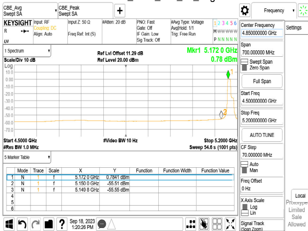
Chain0_5180_106_53_Peak
