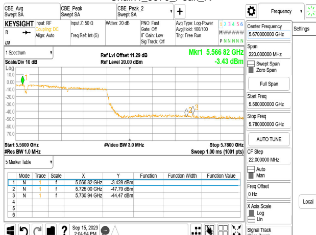
Chain1_5570_Peak_R
