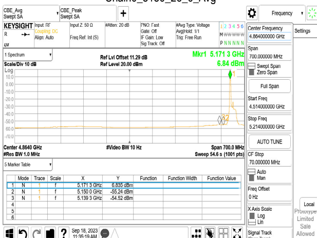
Chain0_5180_26_0_Avg
