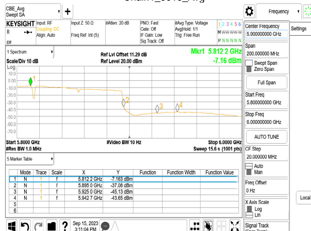
Chain1_5815_Avg
