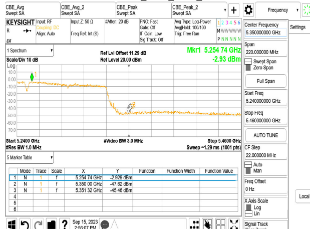
Chain1_5250_Peak_R
