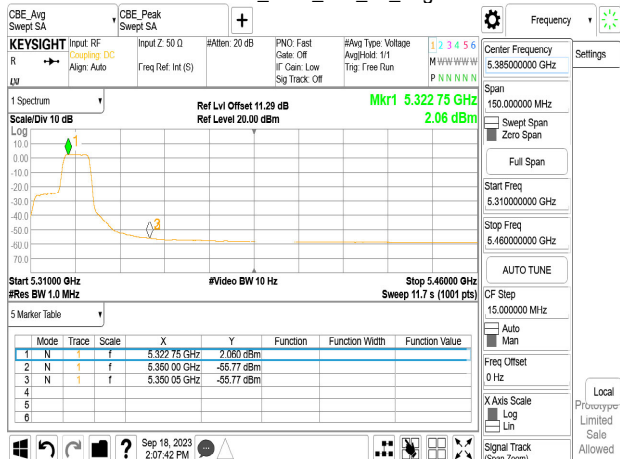
Chain0_5320_106_54_Avg
