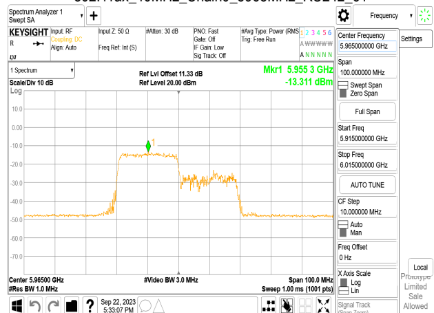
802.11ax_40MHz_Chain0_5965MHz_RU242_61
