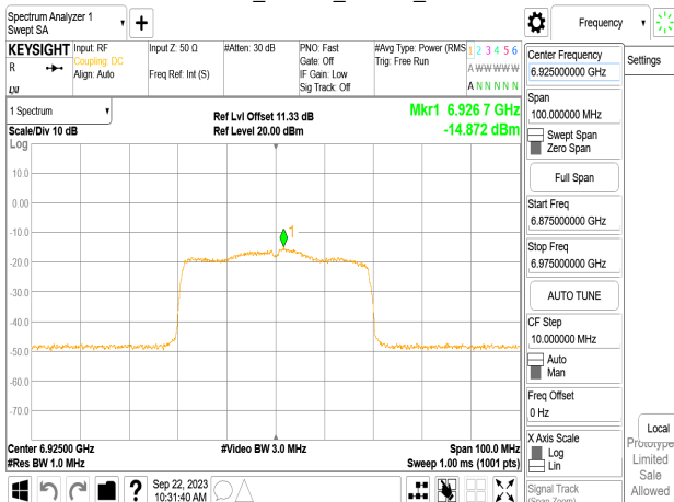
802.11ax_40MHz_Chain0_6925MHz
