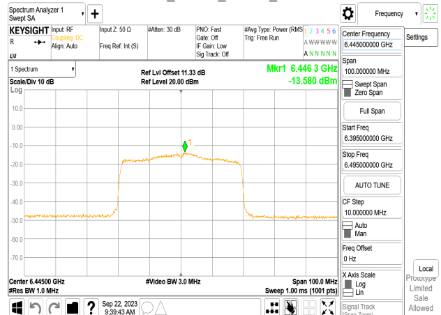
802.11ax_40MHz_Chain0_6445MHz_RU242_61
