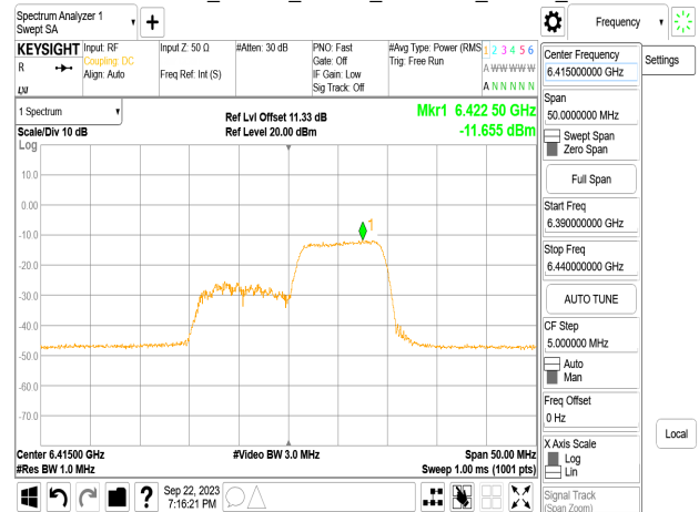
802.11ax_20MHz_Chain1_6415MHz_RU26_8
