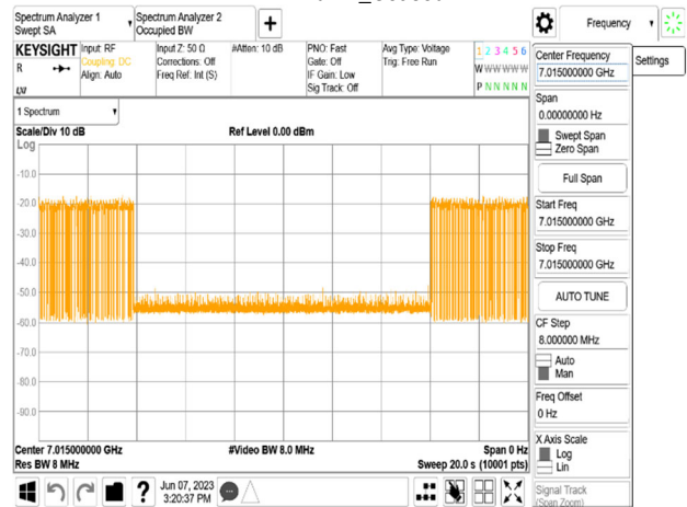
802.11ax_20MHz_CF 7015MHz_Interference_7015MHz_-73.77dBm_Minimal
