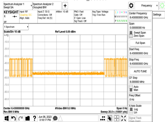
802.11ax_160MHz_CF 6505MHz_Interference_6430MHz_ -71.46dBm_Minimal
