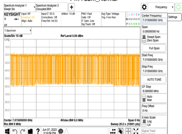
802.11ax_20MHz_CF 7015MHz_Interference_7015MHz_-74.77dBm_Normal
