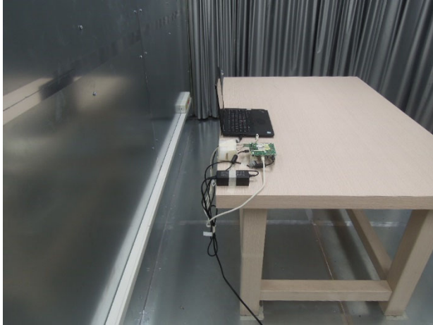
Conduction_Molex_Setup
