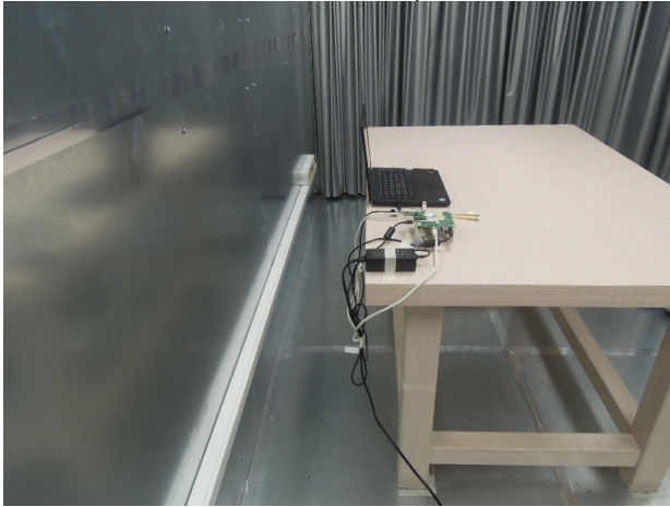
FCC_15_407_WLAN_6E_Conducted_Setup
