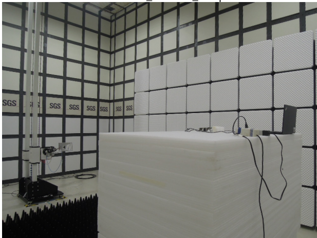
Co-location Radiated Setup
