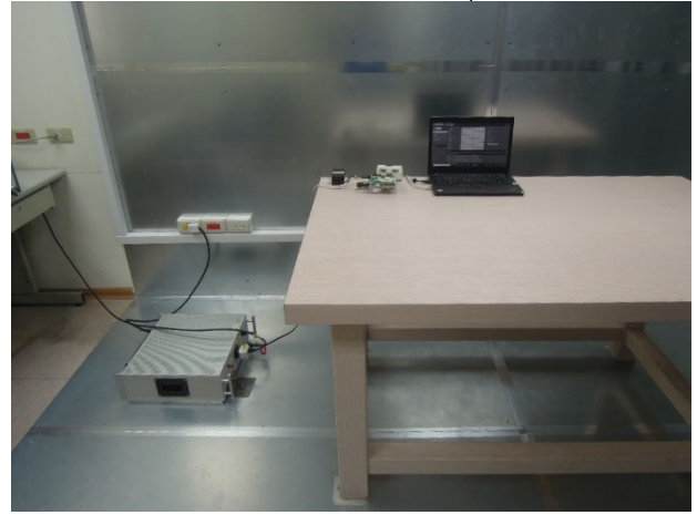
Conduction_UnictronSetup
