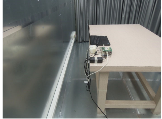
IC_RSS 247_WLAN_Conducted_Setup
