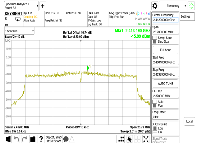
802.11ax_20MHz_Chain1_2412MHz_RU106_53
