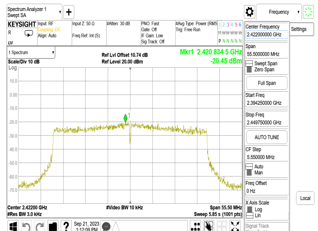
802.11ax_40MHz_Chain1_2422MHz
