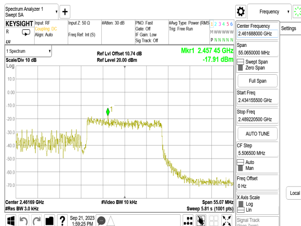
802.11ax_40MHz_Chain1_2452MHz_RU242_62
