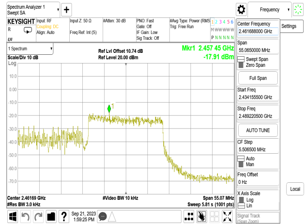
802.11ax_40MHz_Chain1_2452MHz_RU242_62
