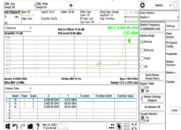
Chain1_5500_Peak
