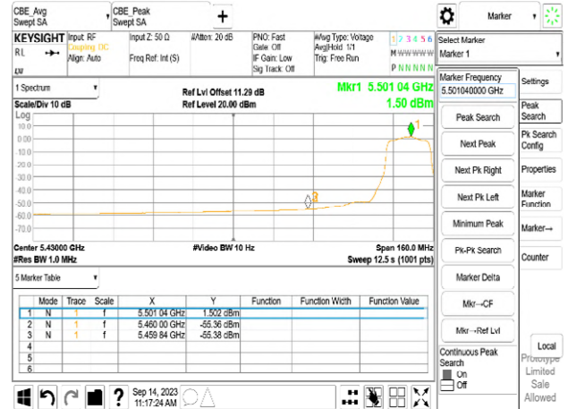
Chain0_5500_Peak
