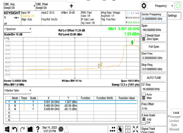
Chain0_5500_Peak
