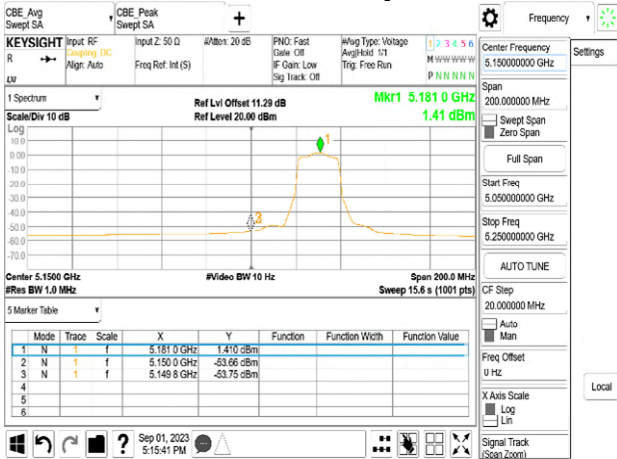
Chain0_5180_Peak
