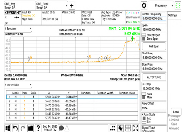
Chain0_5500_Peak
