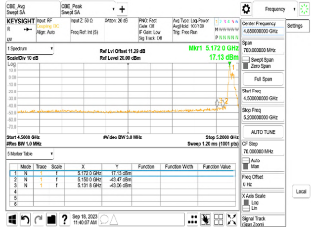
Chain1_5180_52_37_Avg
