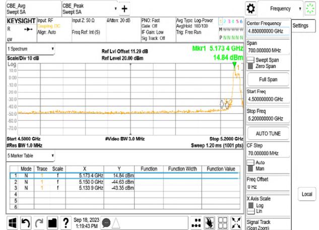
Chain1_5180_52_37_Peak
