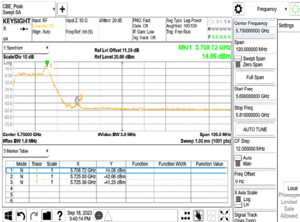
Chain0_5700_52_40_Peak
