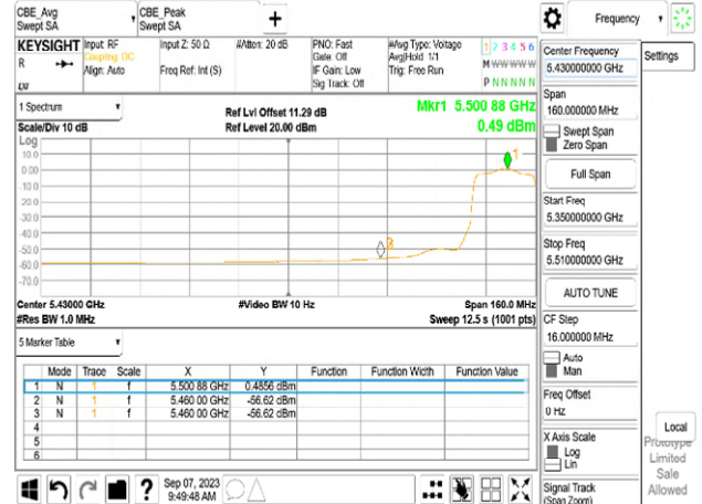
Chain0_500_Peak
