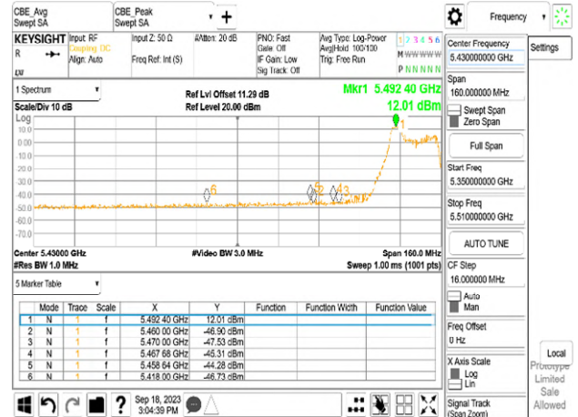
Chain0_500_Avg
