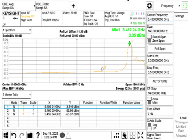
Chain0_500_52_37_Avg
