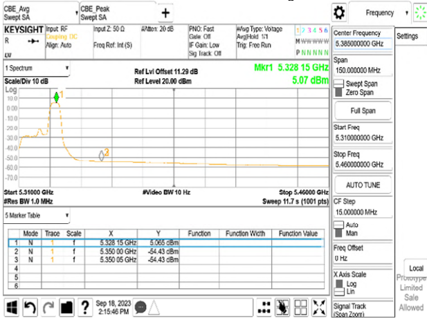
Chain0_5320_52_40_Peak
