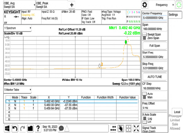
Chain0_5500_106_53_Peak
