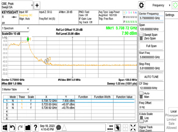
Chain0_5700_26_8_Peak
