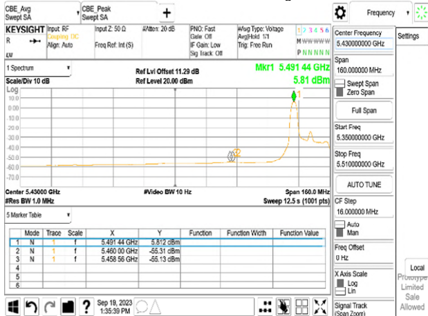
Chain0_500_26_0_Peak
