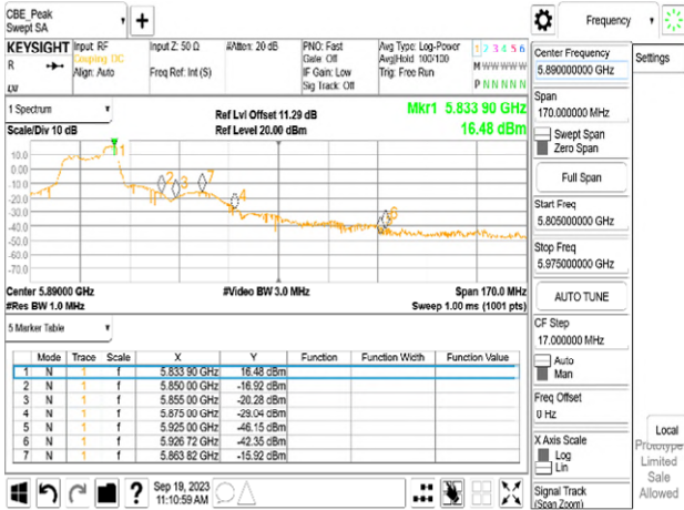
Chain0_5825_Peak
