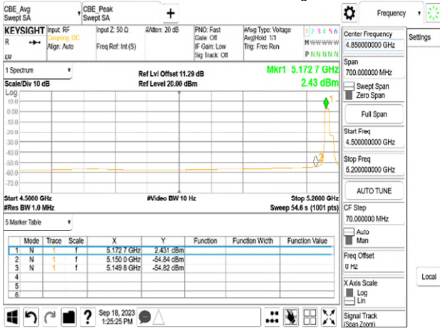
Chain1_5180_106_53_Peak
