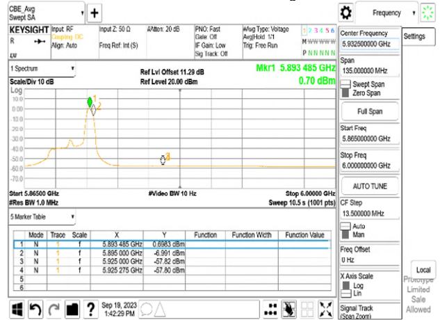
Chain0_5885_52_40_Avg
