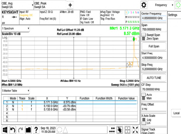
Chain1_5180_26_0_Avg
