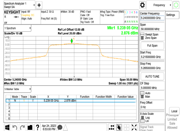
802.11ax_20MHz_Chain1_5240MHz_RU106_53
