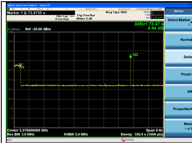
Radar at end of CAC - 5570MHz
