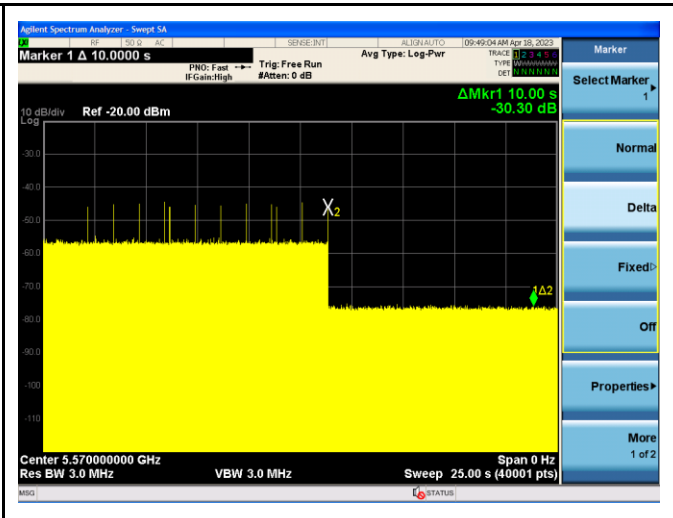
Channel Move Time - 5570MHz (Type5)
