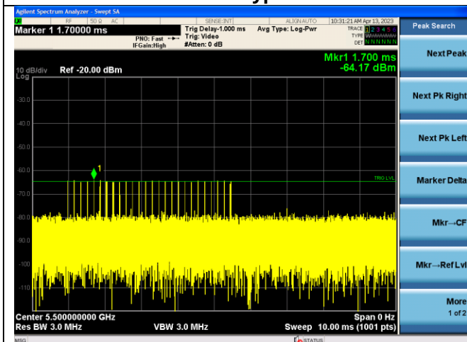
Radar Type 2
