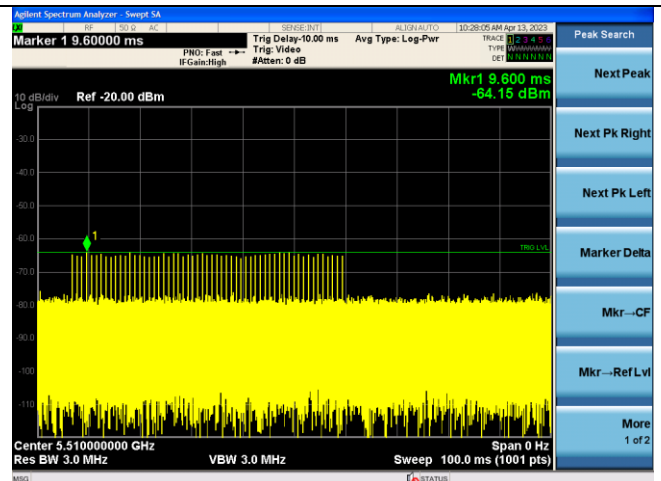
Radar Type 1
