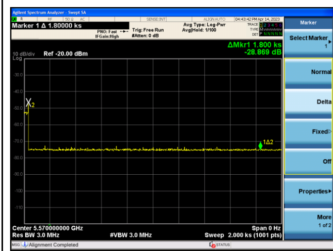
Non-Occupancy Period - 5570MHz
