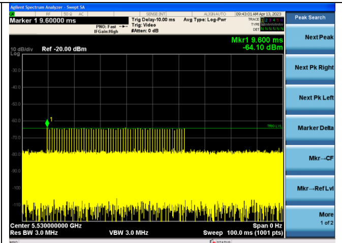
Radar Type 1
