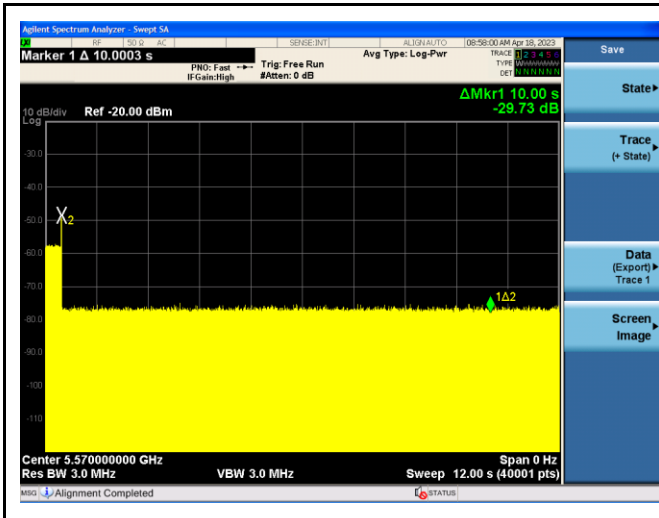
Channel Move Time - 5570MHz (Type0)
