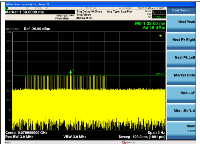
Radar Type 1
