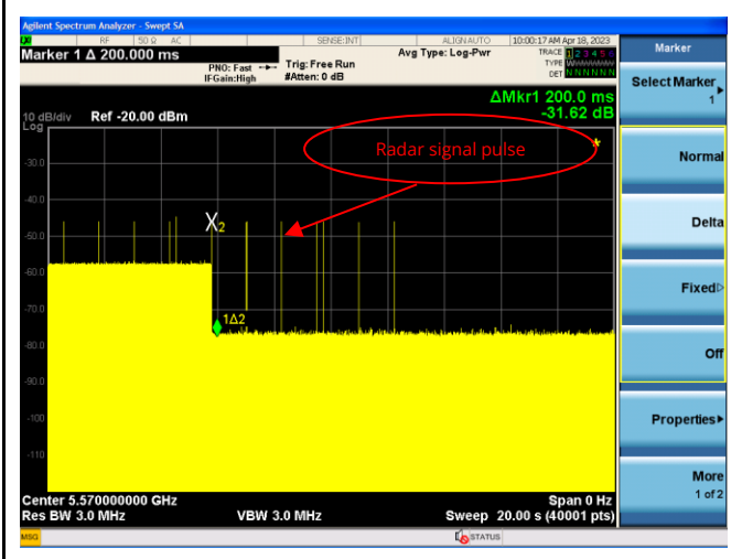
Channel Closing Time - 5570MHz (Type5)
