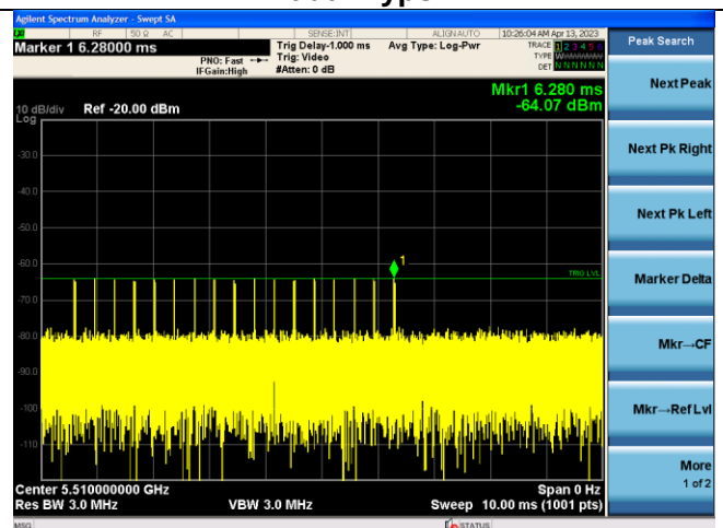
Radar Type 3
