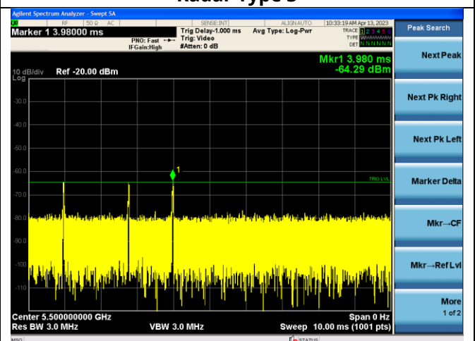
Radar Type 5
