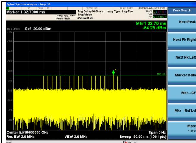
Radar Type 0
