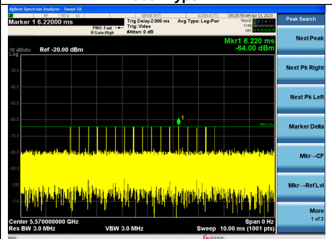
Radar Type 3
