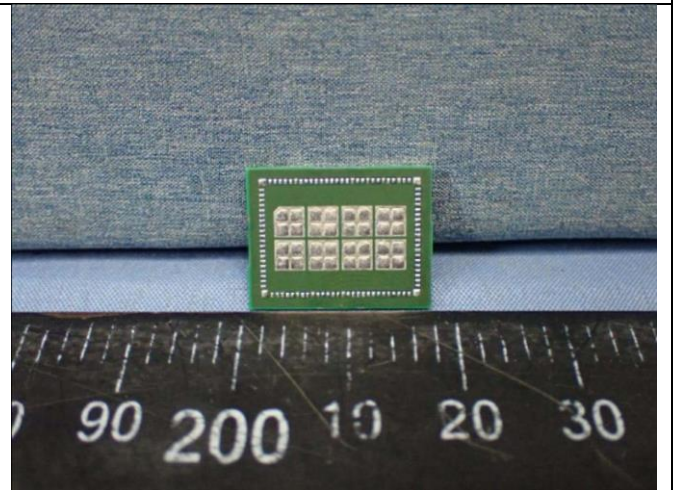
EUT Bottom View (without interface card)
