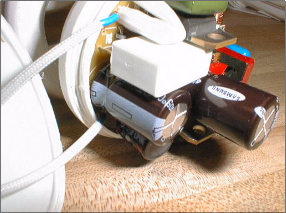
New capacitor C1 shown in side view.
