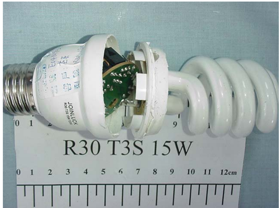
FIGURE 1 ENERGY SAVING LAMP (M/N: R30 T3S 15W) COVER REMOVED
