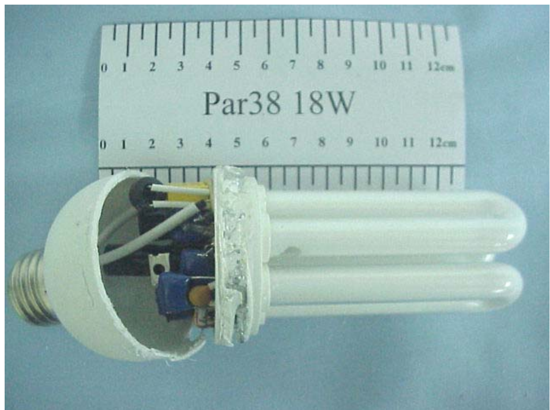
FIGURE 2 ENERGY SAVING LAMP (M/N: Par38 18W) COVER REMOVED 2
