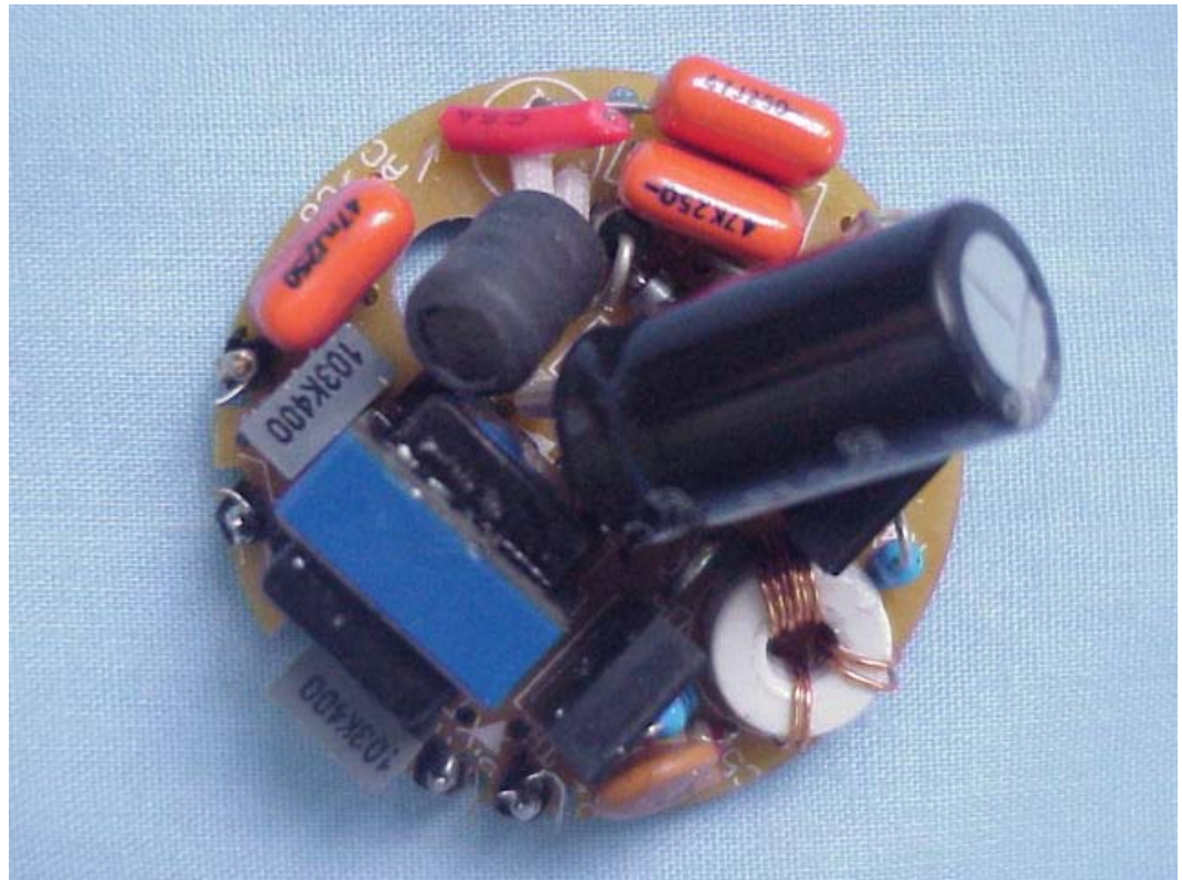
FIGURE 5 ELECTRONIC ENERGY SAVING LAMP (M/N: JLC7-18 REFLECTOR 11W) MAIN BOARD (COMPONENT SIDE)
