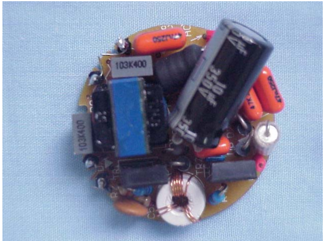
FIGURE 2 ELECTRONIC ENERGY SAVING LAMP (M/N: JLC7-18 A-TYPE 11W) MAIN BOARD (COMPONENT SIDE)
