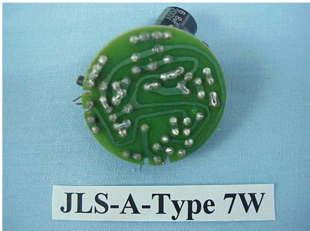
FIGURE 3 ELECTRONICS ENERGY SAVING LAMP (M/N: JLS A-TYPE 7W) MAIN BOARD (SOLDERED SIDE)
