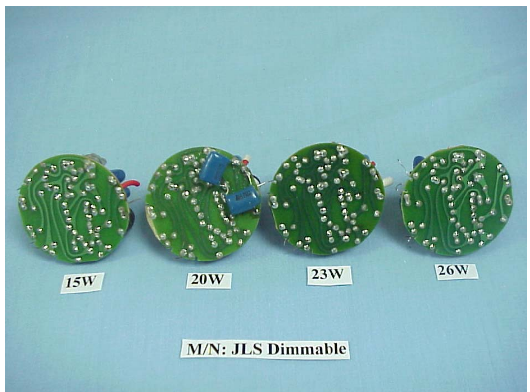
FIGURE 3 ELECTRONIC ENERGY SAVING LAMP (M/N: JLS DIMMABLE 15W/20W/23W/26W) MAIN BOARD (SOLDERED SIDE)
