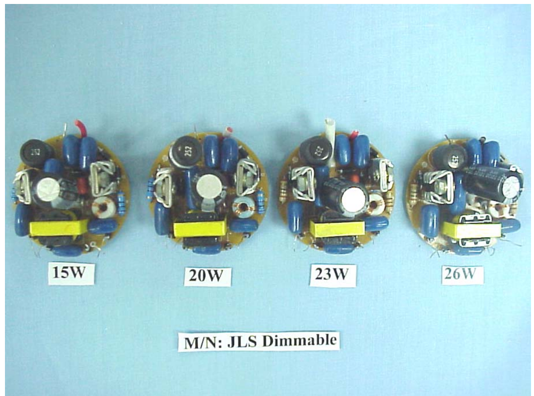
FIGURE 2 ELECTRONIC ENERGY SAVING LAMP (M/N: JLS DIMMABLE 15W/20W/23W/26W) MAIN BOARD (COMPONENT SIDE)
