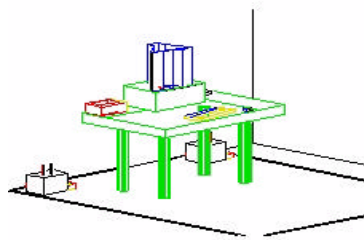
Figure 4. Wooden Table & Bonded LISNs
