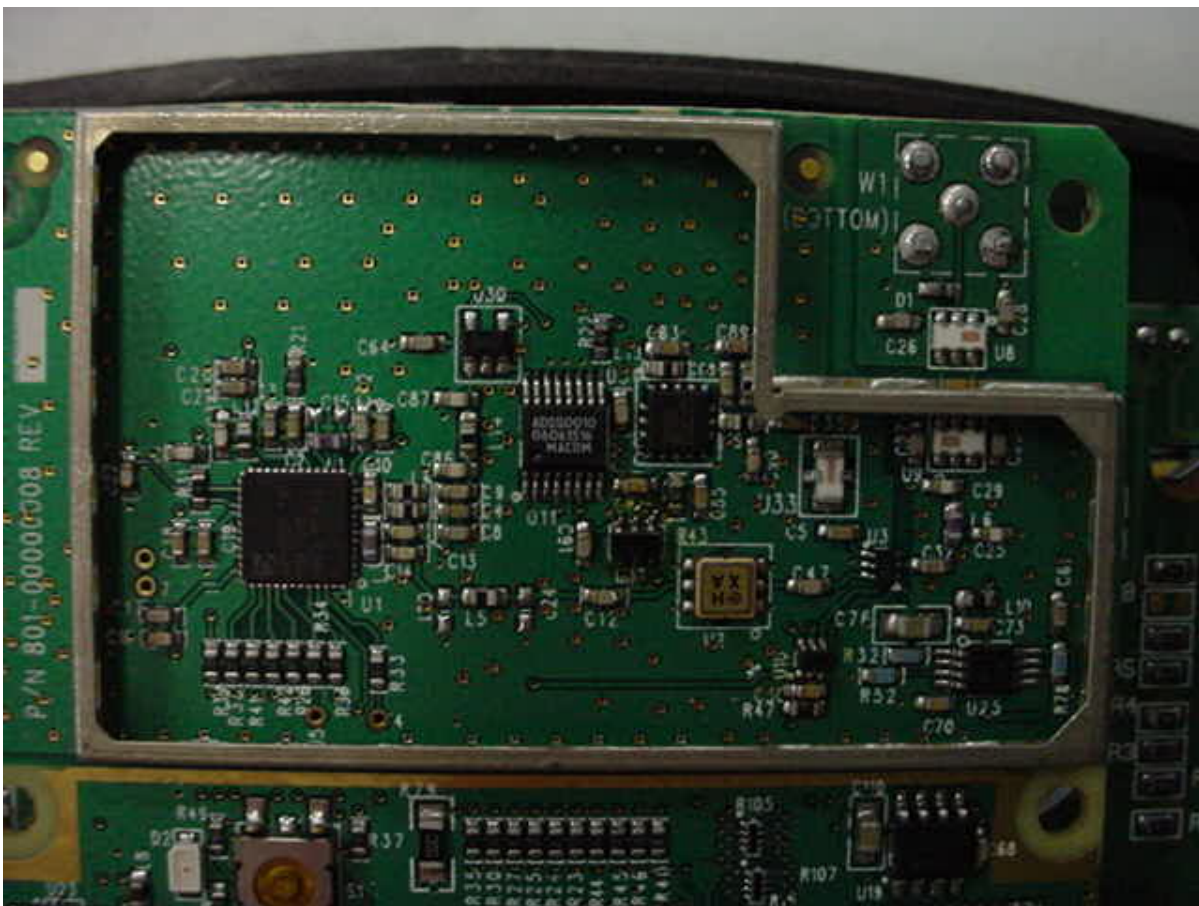
Photo Three – Internal RF Section – Shield Removed
