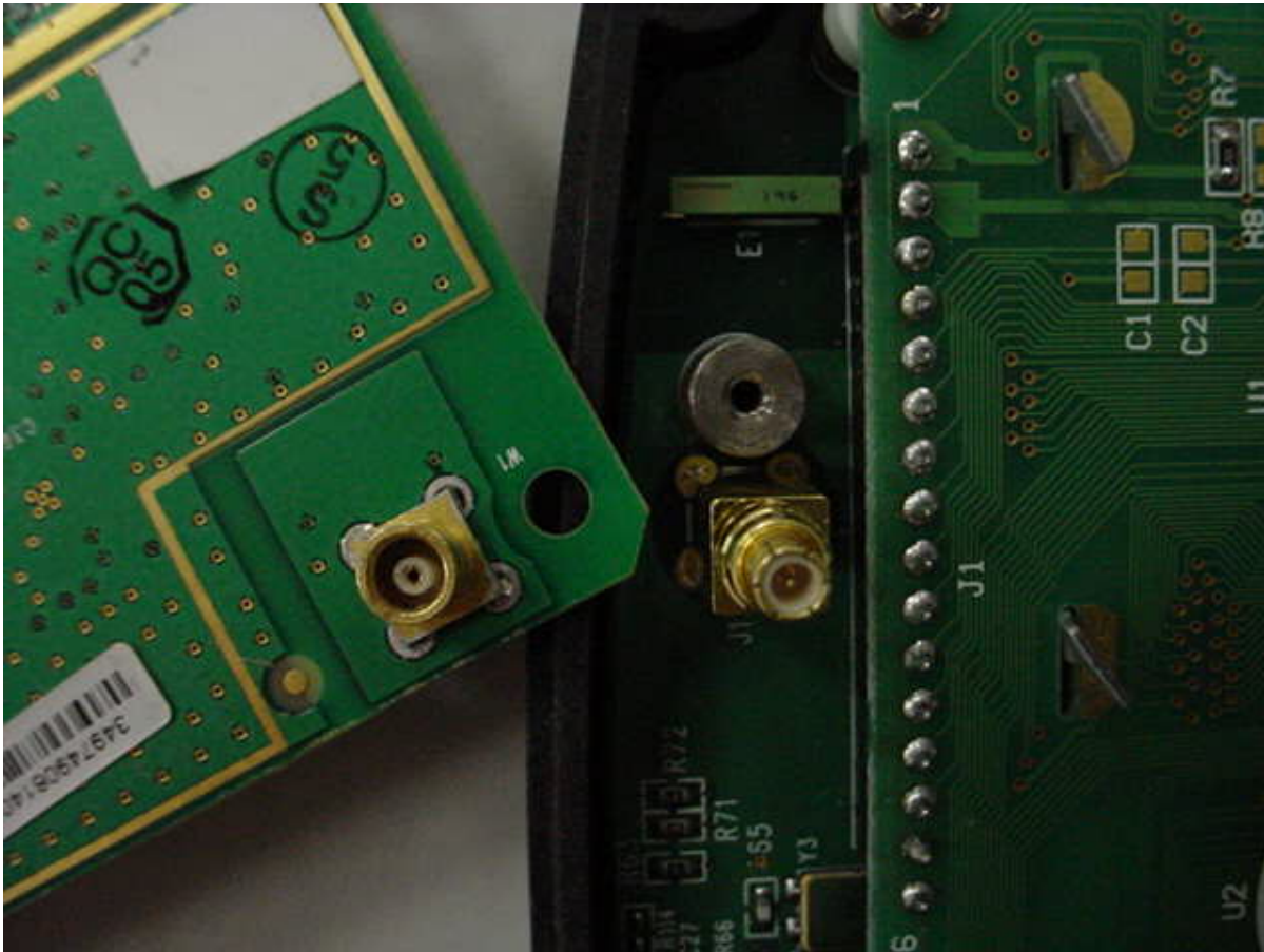
Photo Five – Internal View Showing Antenna Connectors
