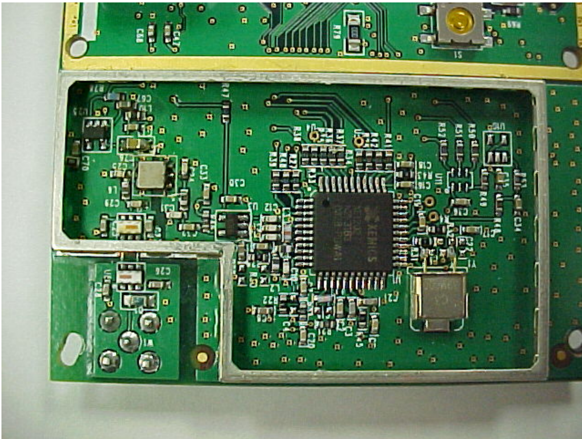
Photo Two – Internal RF Section, Component Side, Shield Removed
