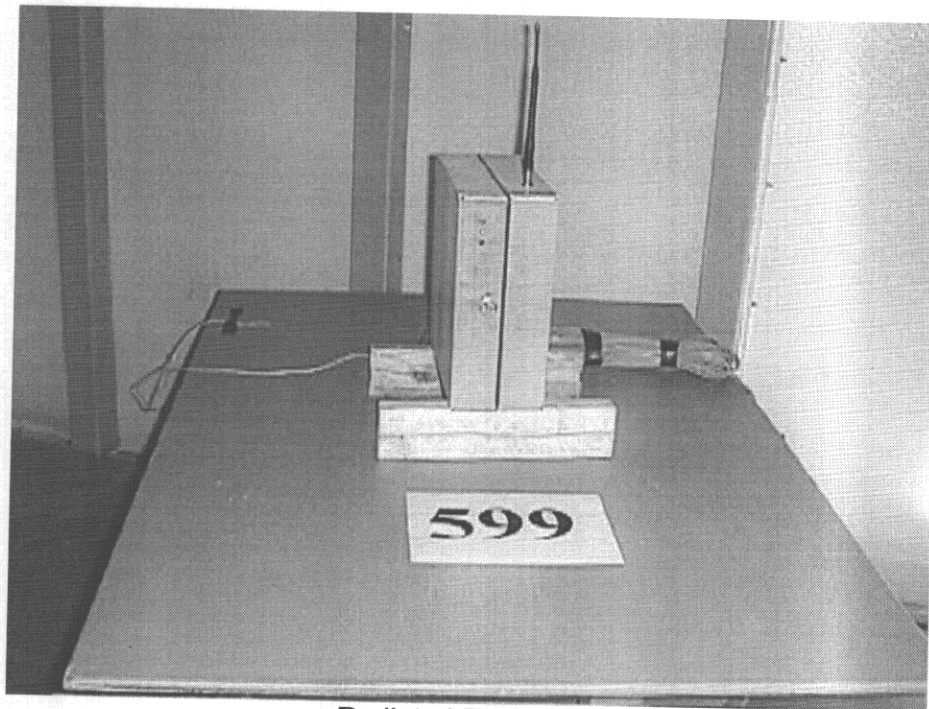
Radiated Emissions
