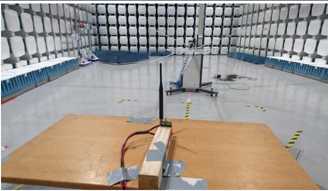
Radiated emission 30MHz - 1 GHz with dipole antenna
