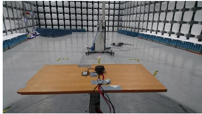
Radiated emission 30MHz - 1 GHz with monopole antenna
