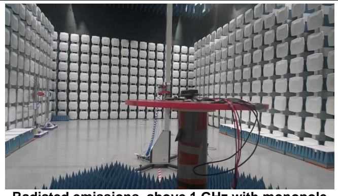
Radiated emissions above 1 GHz with monopole antenna
