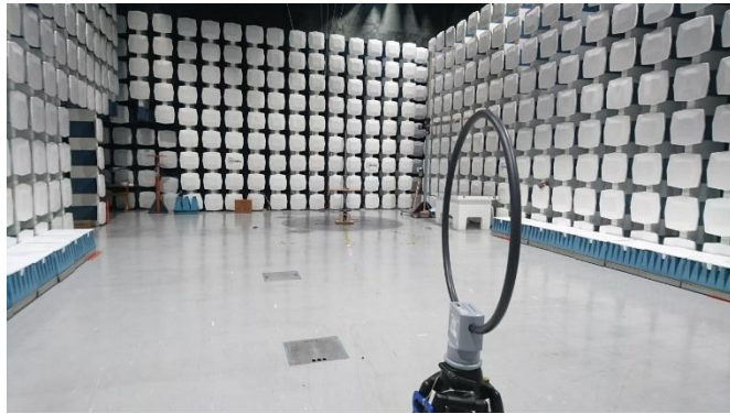
Radiated emissions below 30MHz
