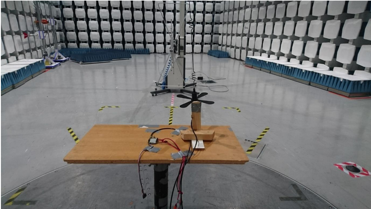
Radiated emission 30MHz - 1 GHz
