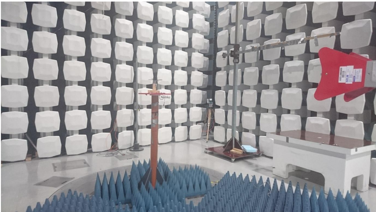
Radiated emissions 1 GHz - 10 GHz
