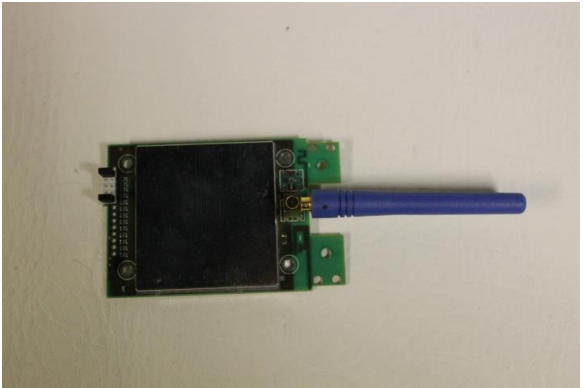
Photograph 3. setup1, without power supply
