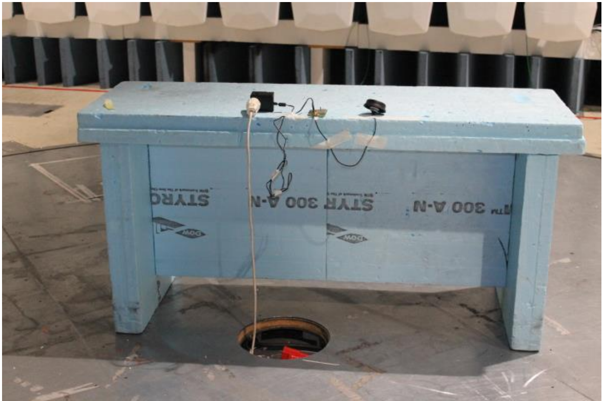
Photograph 1. Spurious radiated emissions test setup (setup4)
