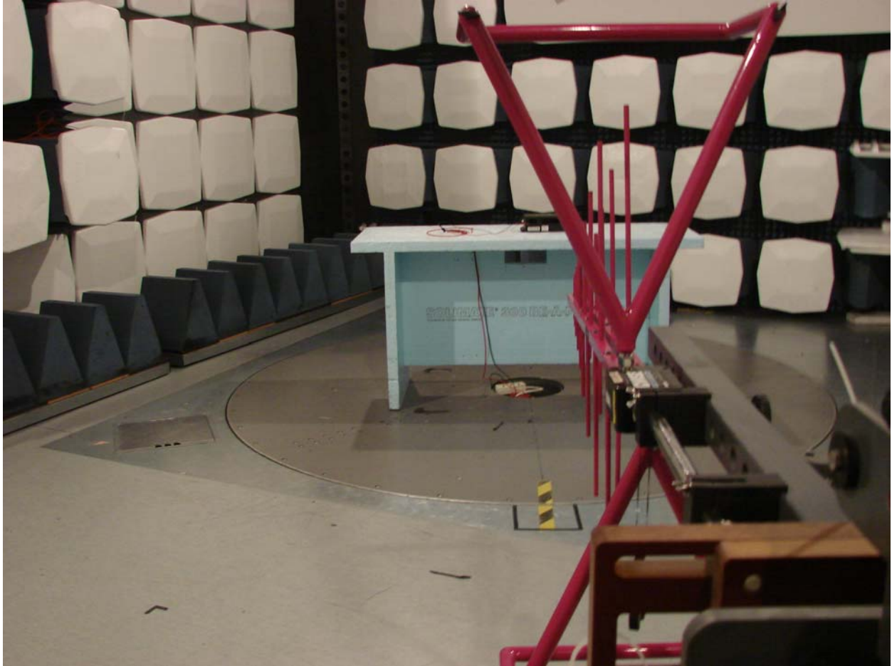
Picture 1: Receiver Radiated emission test setup <1 GHz
