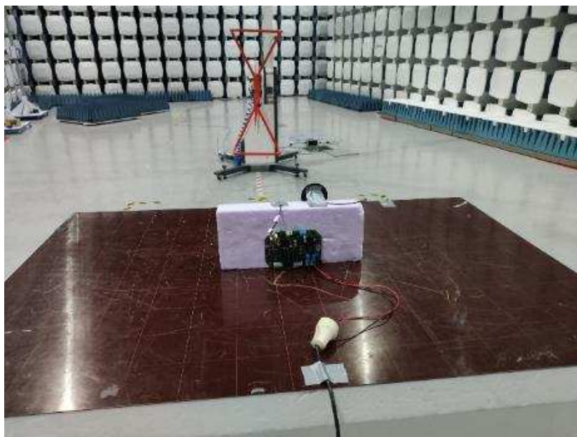
Radiated Emissions 30 – 1000 MHz
