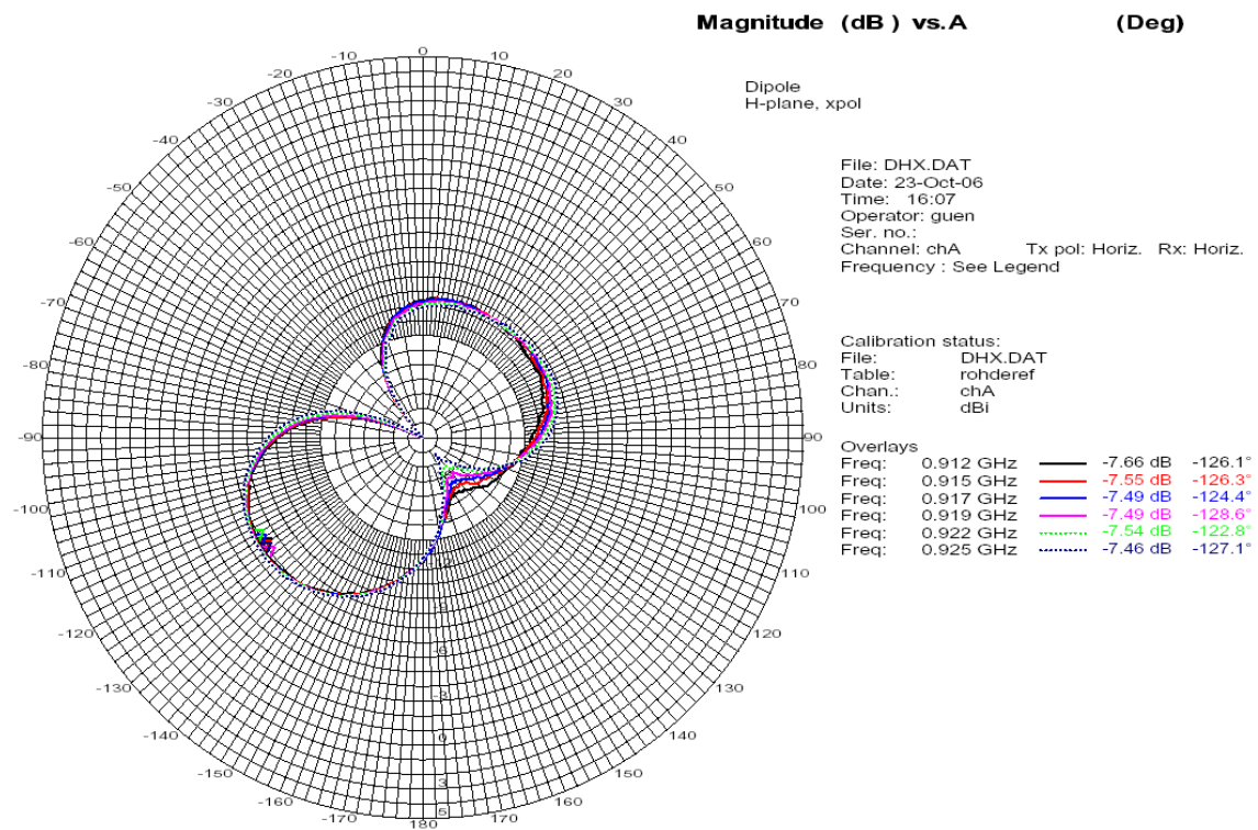
Fig 4: Dipole, H-plane, xpol (horizontal pol)
