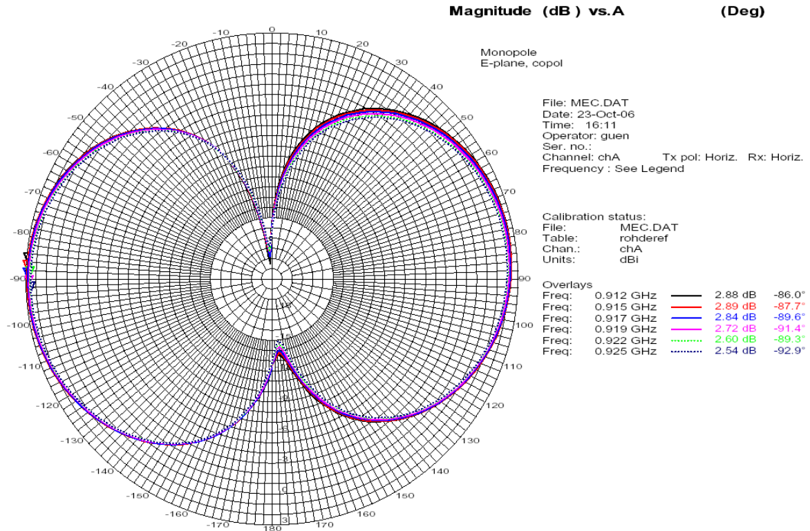
Fig 5: Monopole, E-plane, copol (horizontal pol)
