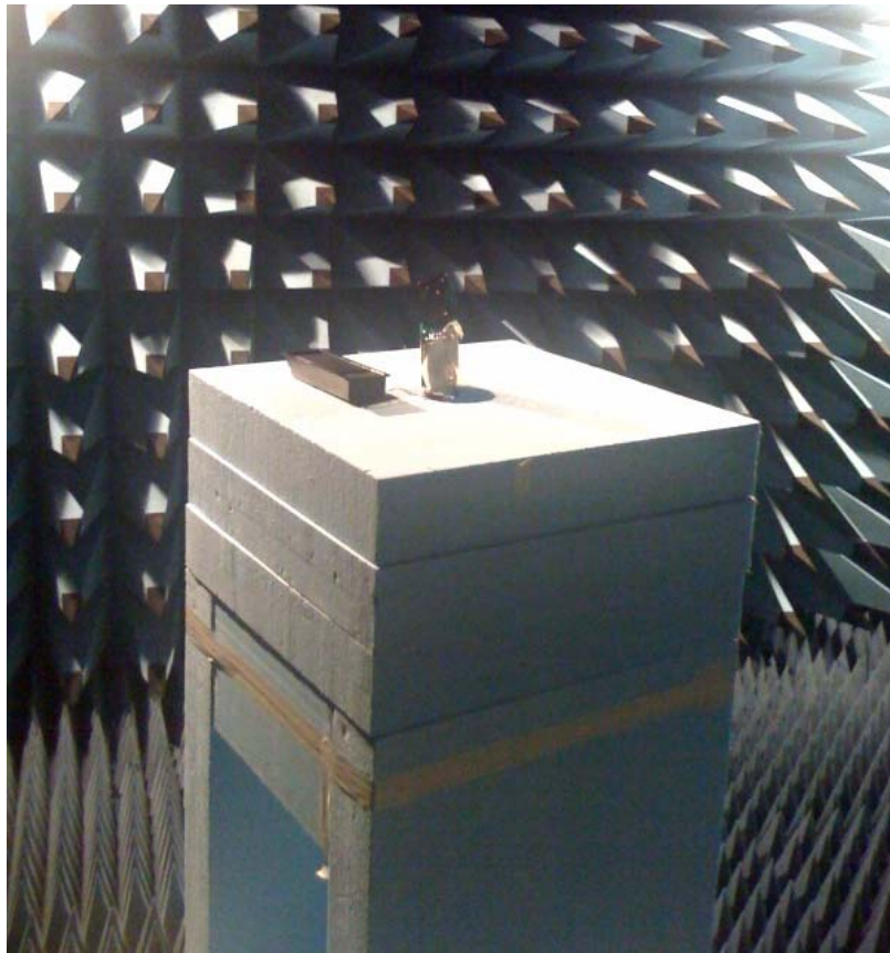
Radiated spurious emission 1-5 GHz
