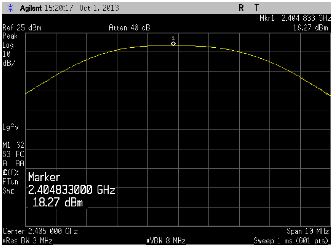
Figure 1, channel 0, conducted peak output power
