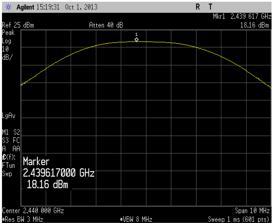
Figure 2, channel 7, conducted peak output power
