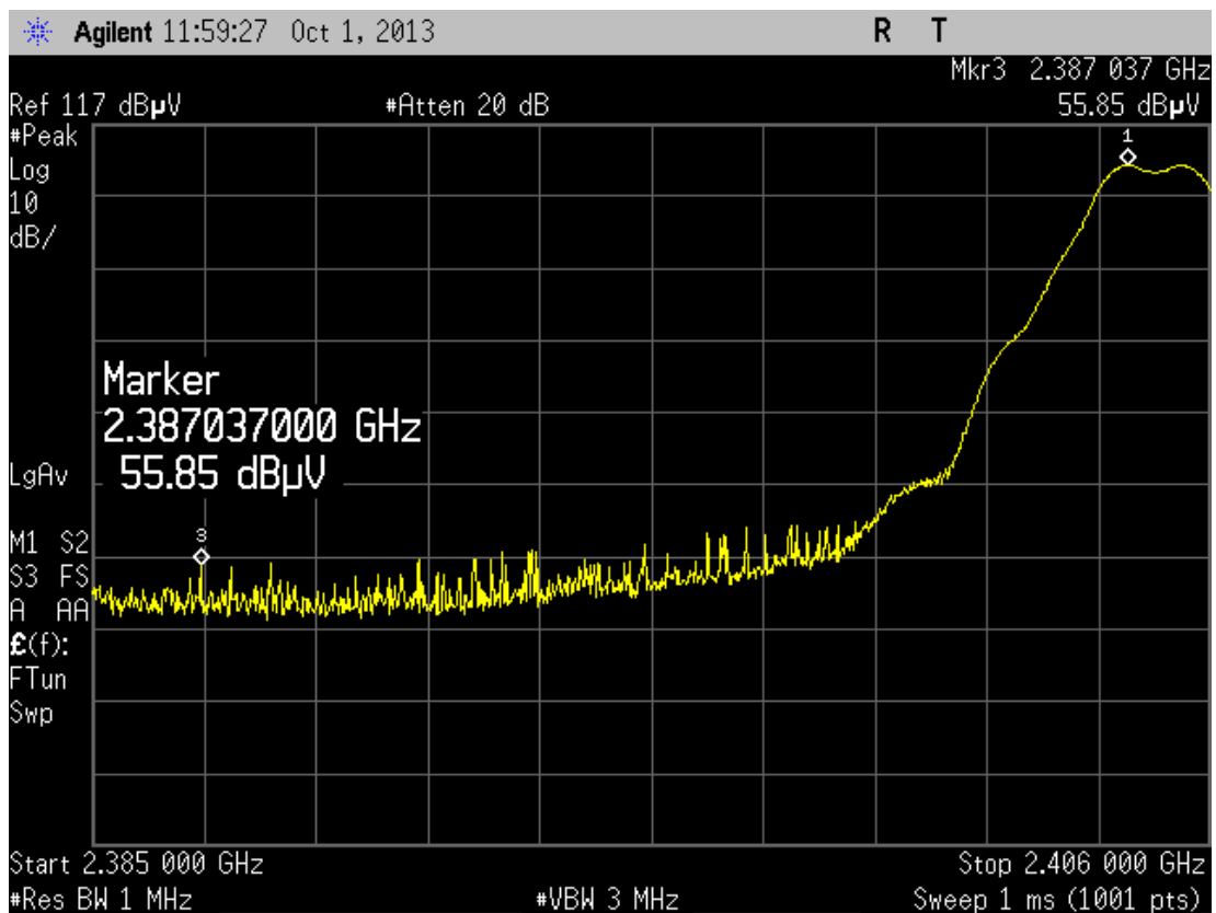
Figure 11, Hopping on, Band-edge compliance, low end <2390MHz
