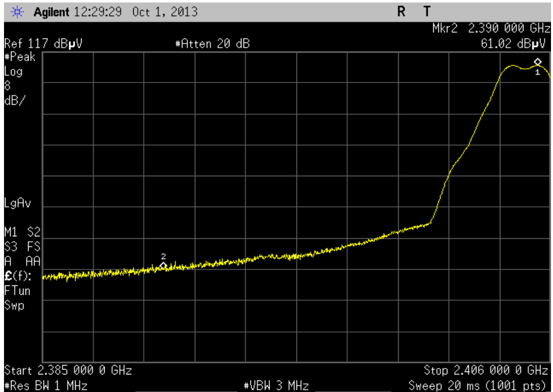
Figure 8, Hopping off, Channel 0, Band-edge compliance, low end
