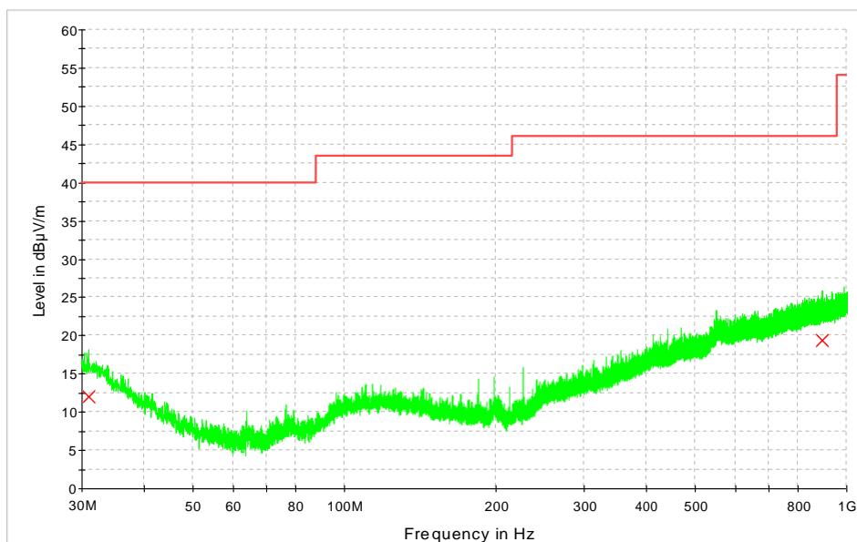
Figure 16, Spurious emissions, 30-1000 MHz, middle channel
