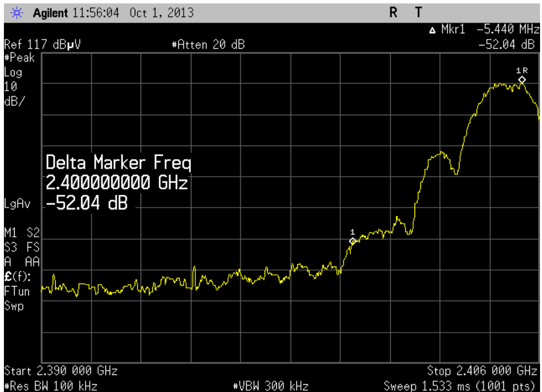
Figure 10, Hopping on, Band-edge compliance, low end <2400MHz
