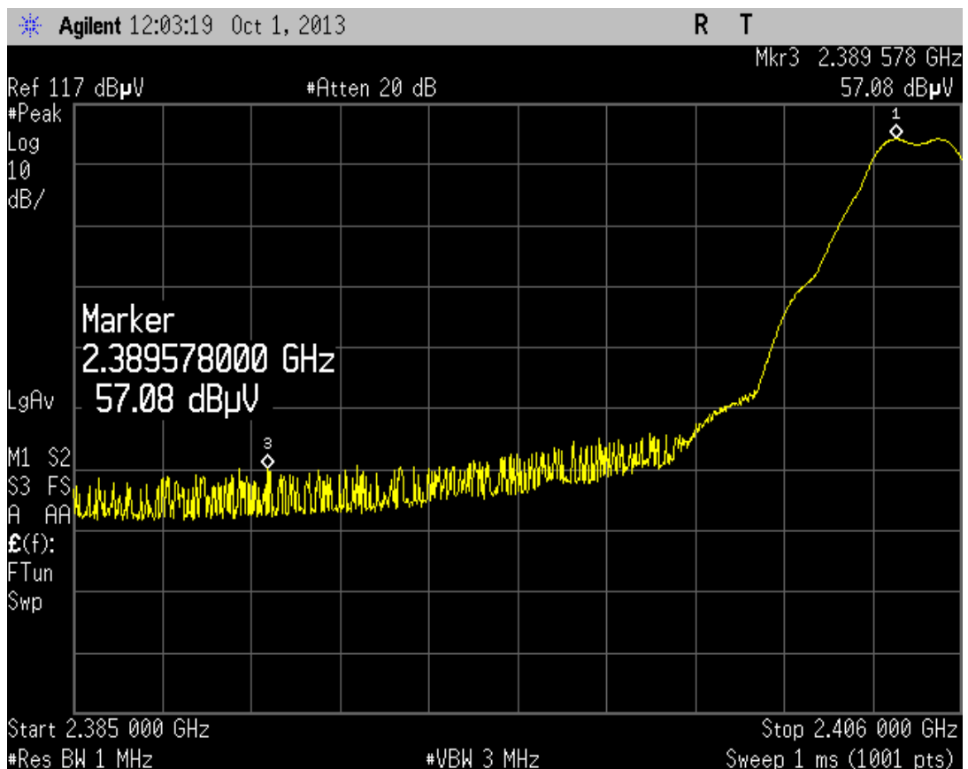
Figure 13, Hopping off, Channel 0, Band-edge compliance, low end
