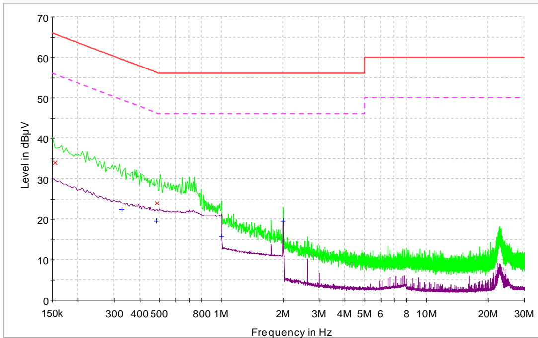
Figure 10. AC powerline emissions, Line N
