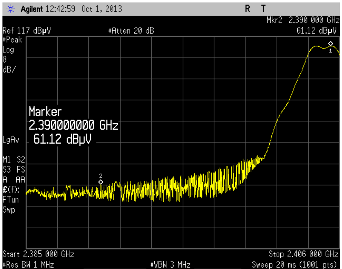
Figure 5, Hopping on, Band-edge compliance, low end <2390MHz
