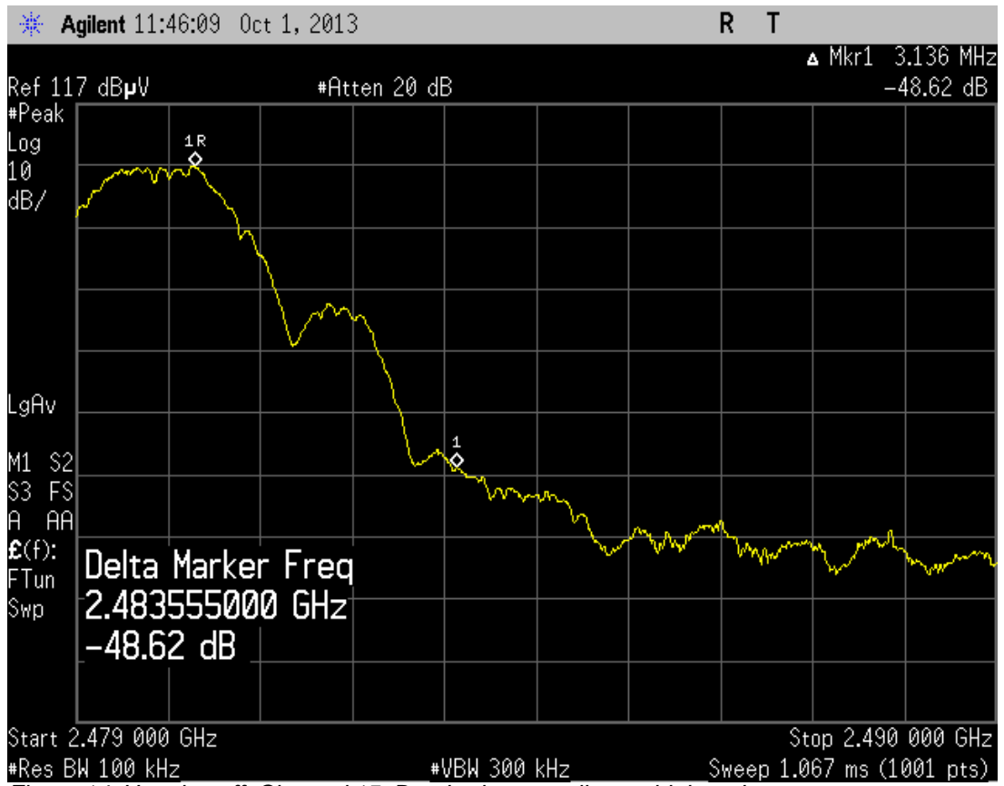
Figure 14, Hopping off, Channel 15, Band-edge compliance, high end
