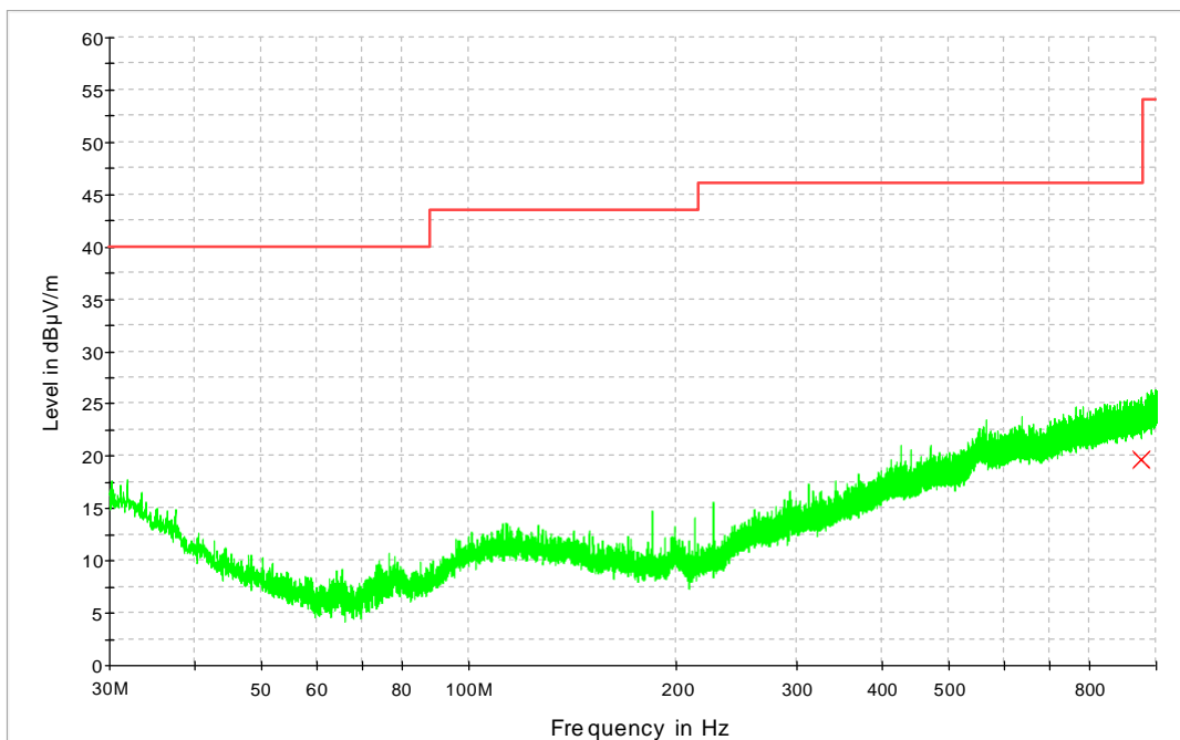
Figure 15, Spurious emissions, 30-1000 MHz, middle channel
