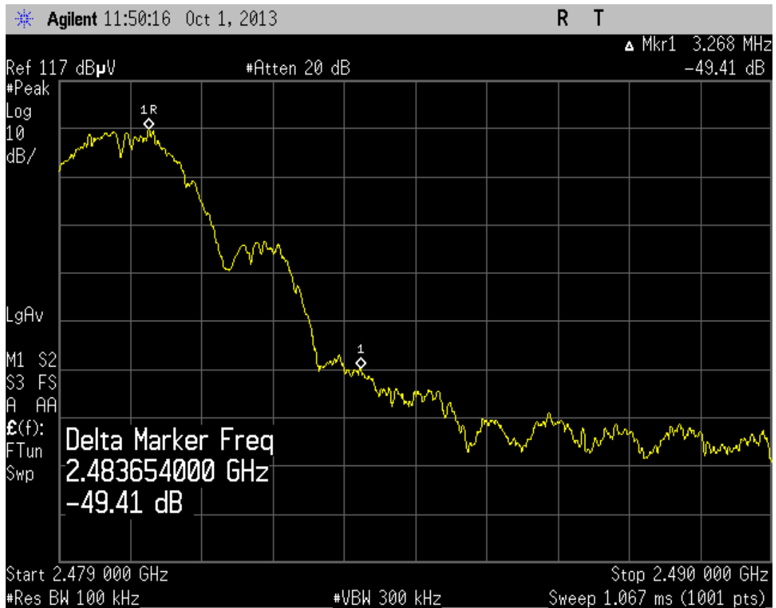
Figure 12, Hopping on, Band-edge compliance, high end
