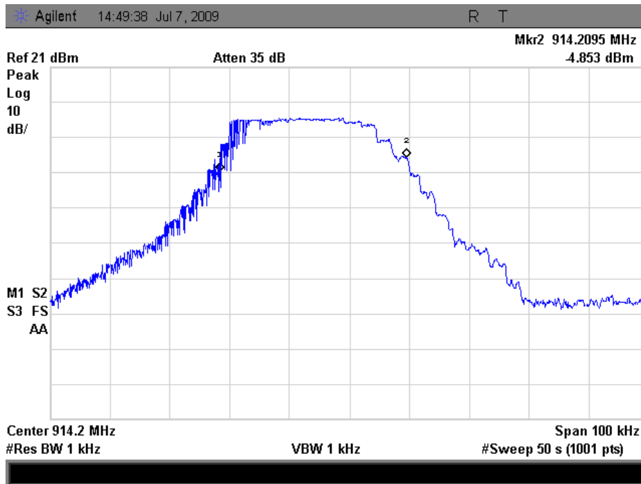
Picture 28: 99% Bandwidth measurement result; middle channel
