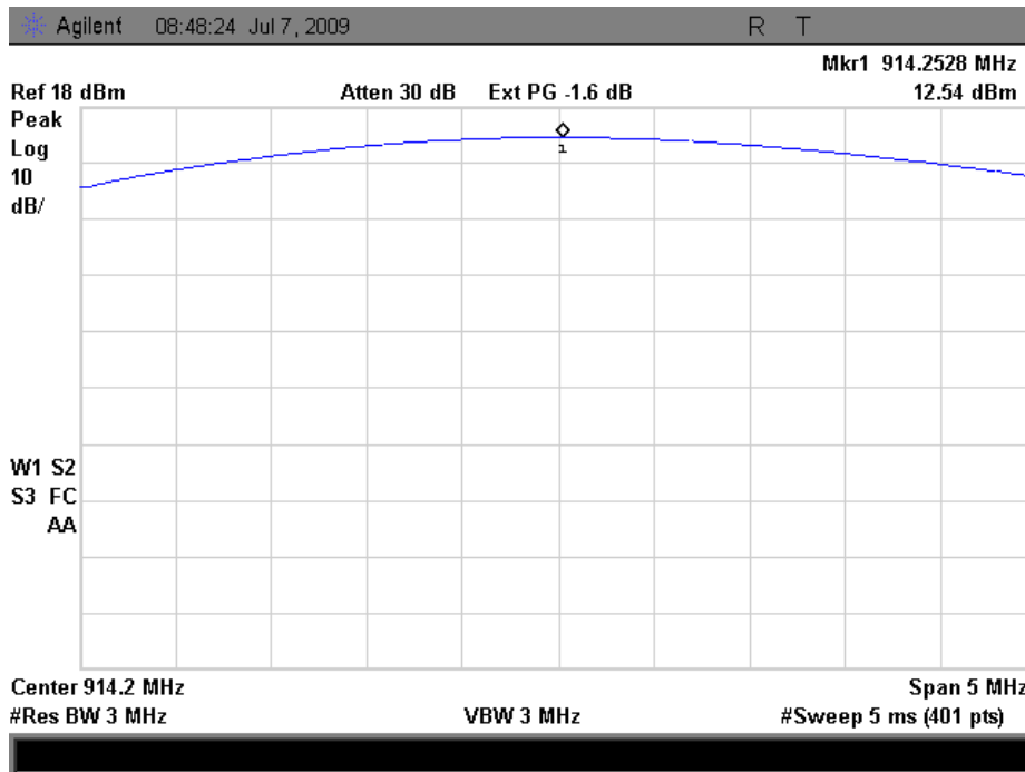
Picture 14: Peak output power, middle channel
