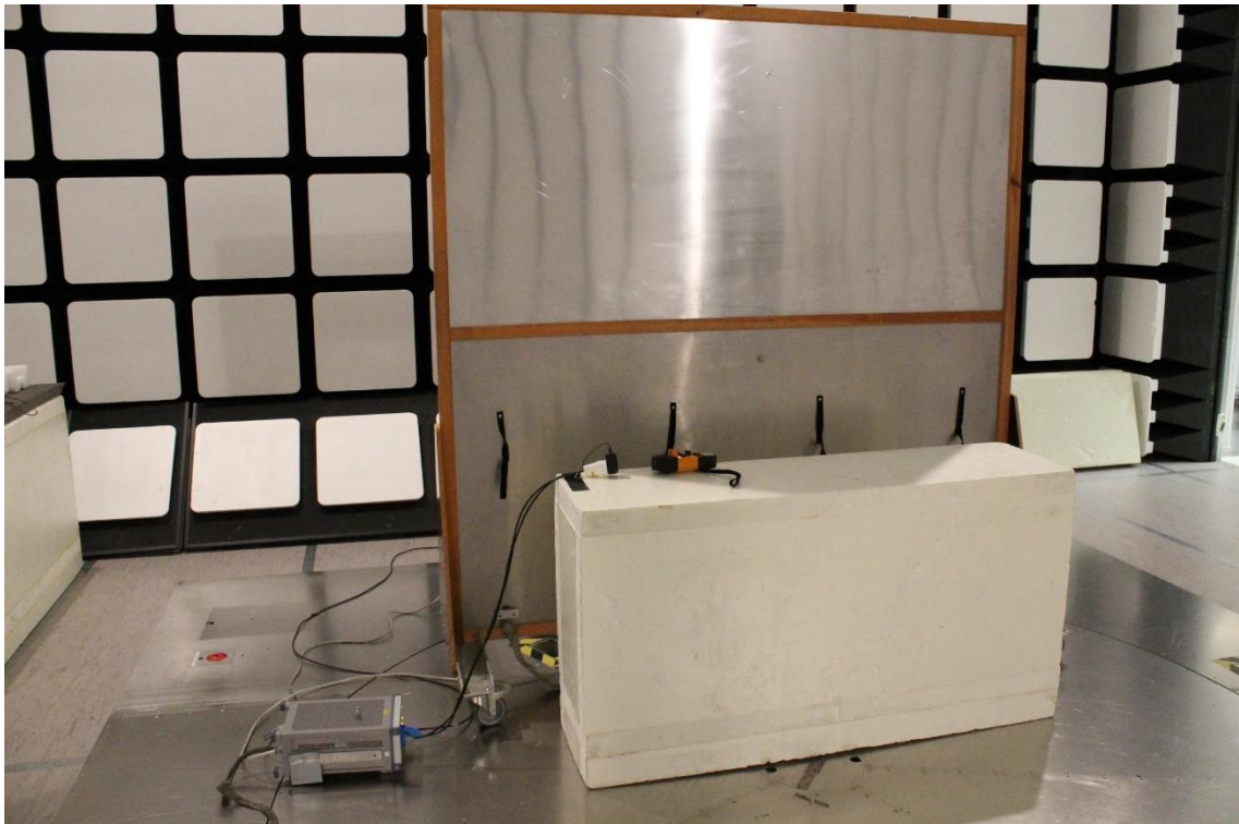
Photograph 12. Conducted Emissions
