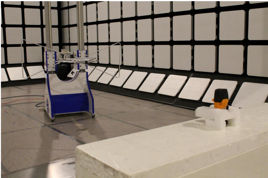
Photograph 8. Radiated Spurious Emissions 30 MHz – 1000 MHz
