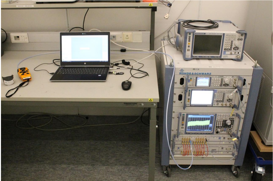
Photograph 13. FCC Conducted measurements
