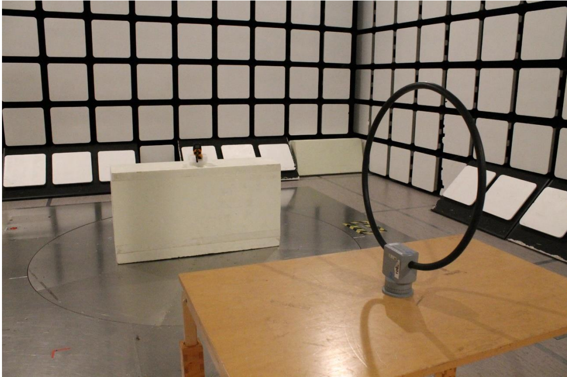
Photograph 7. Radiated Spurious Emissions 9 kHz – 30 MHz
