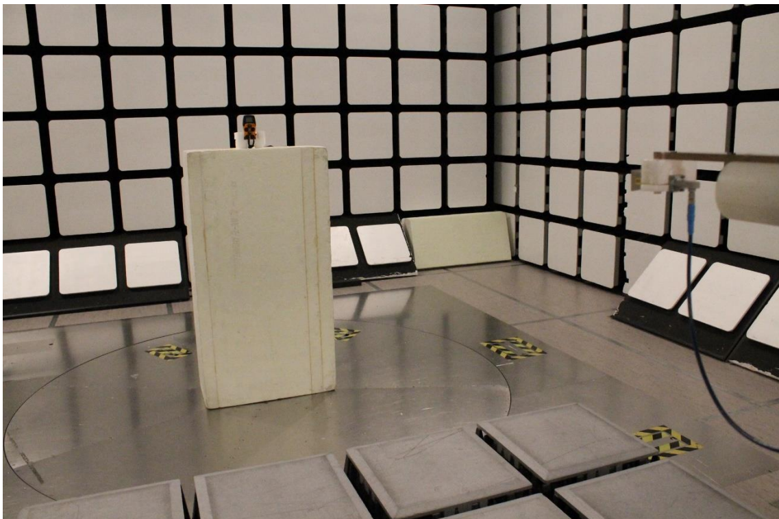
Photograph 10. Radiated Spurious Emissions 18 GHz – 26.5 GHz
