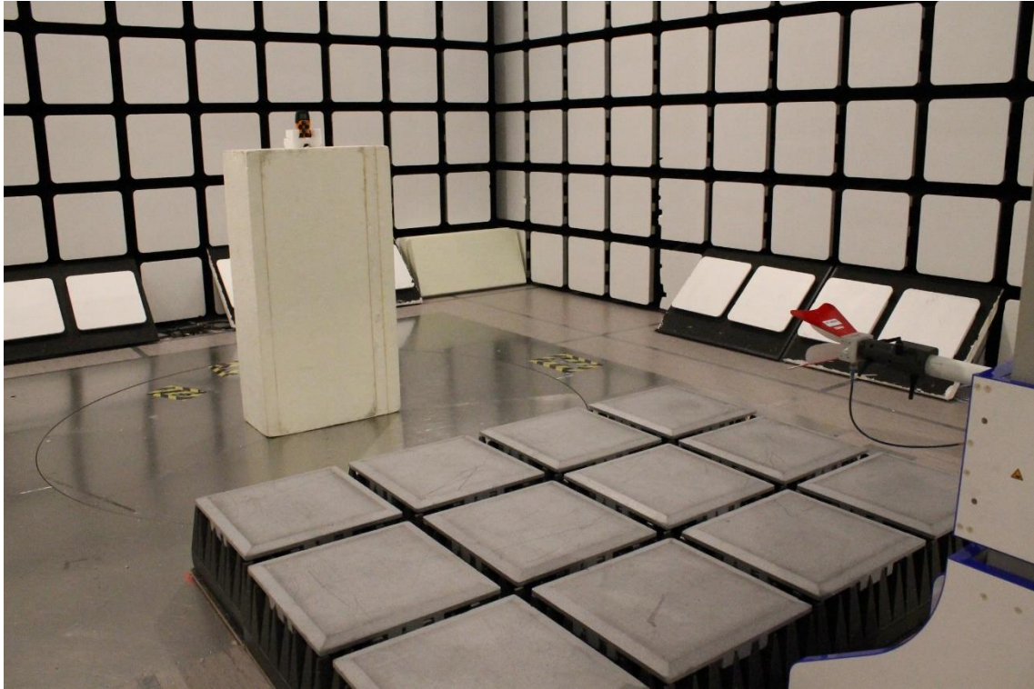
Photograph 9. Radiated Spurious Emissions 1 GHz – 18 GHz
